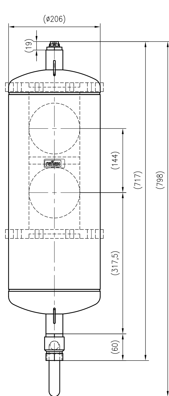
Side view
