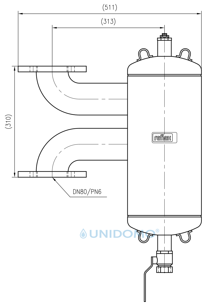
Front view
