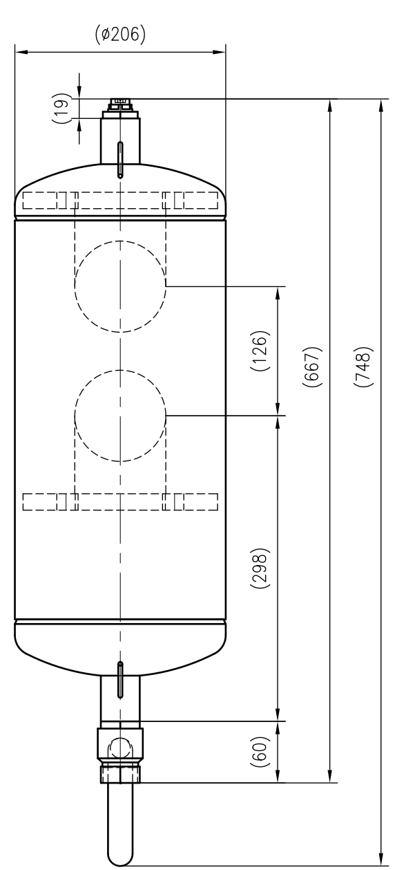
Side view
