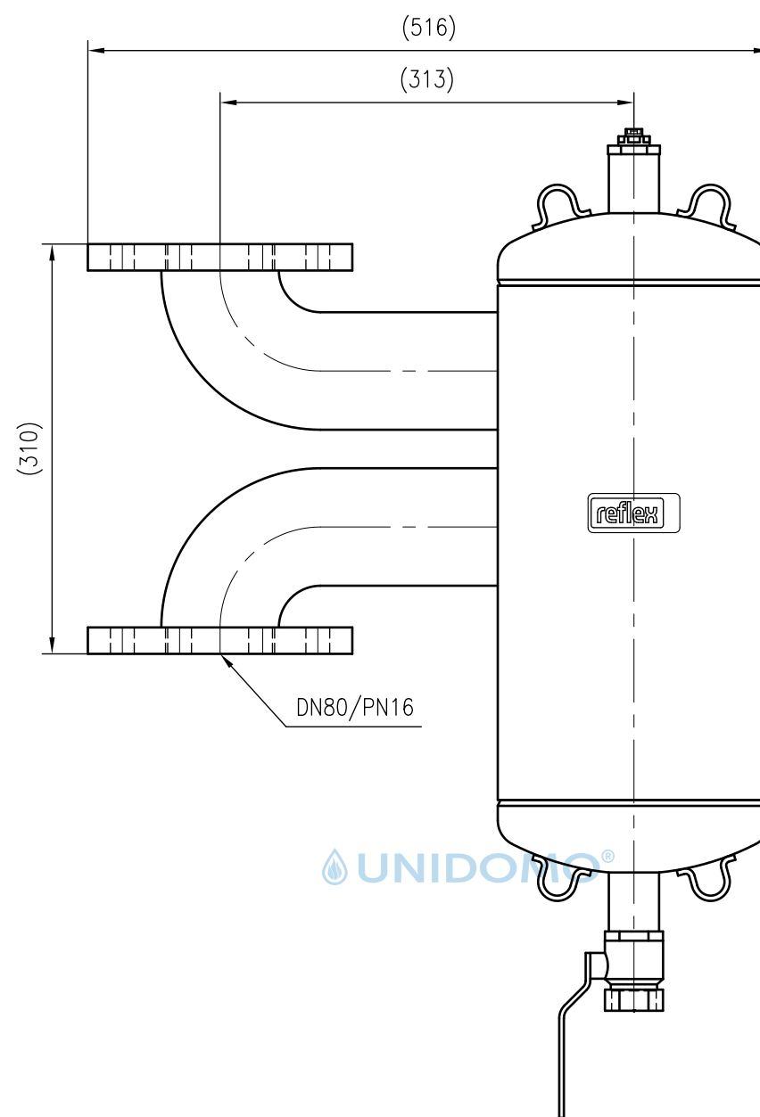
Front view
