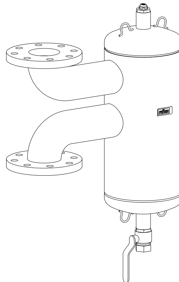
Isometric view
