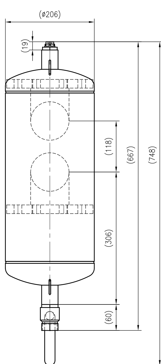
Side view
