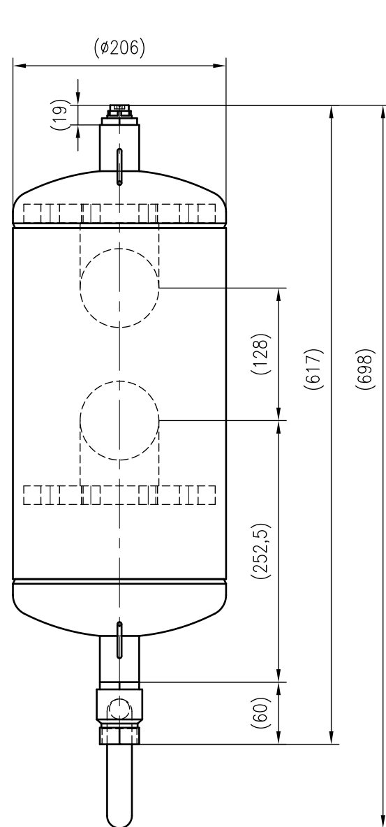
Side view
