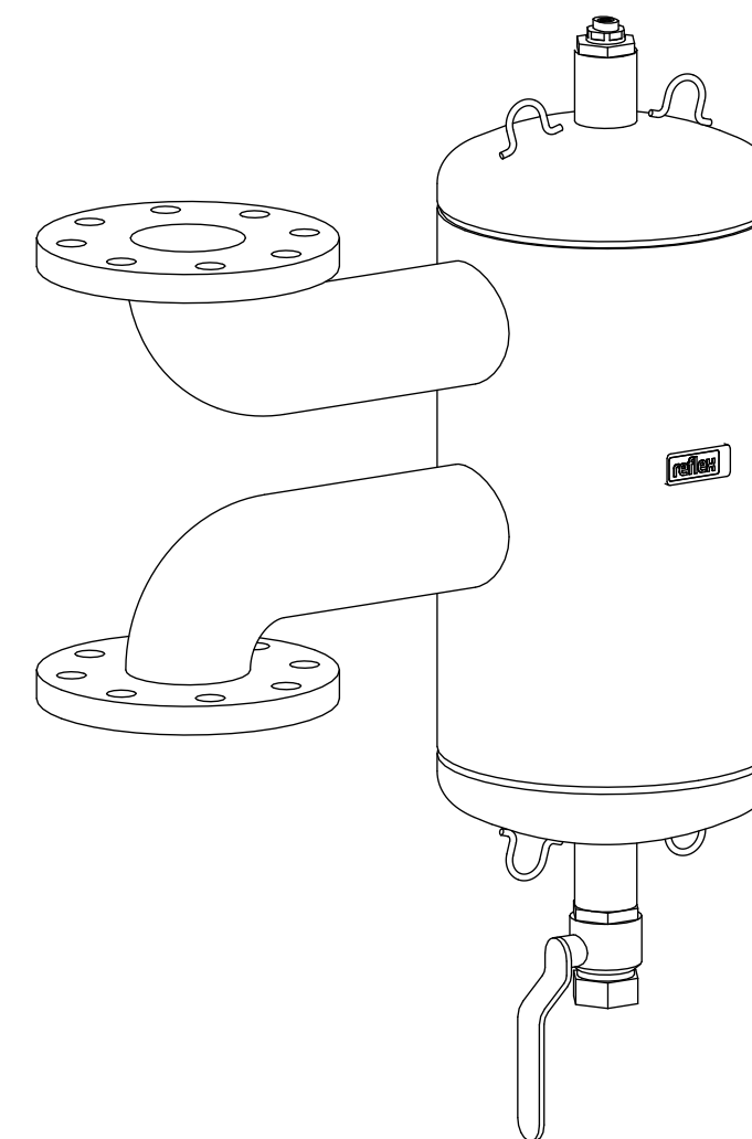
Isometric view
