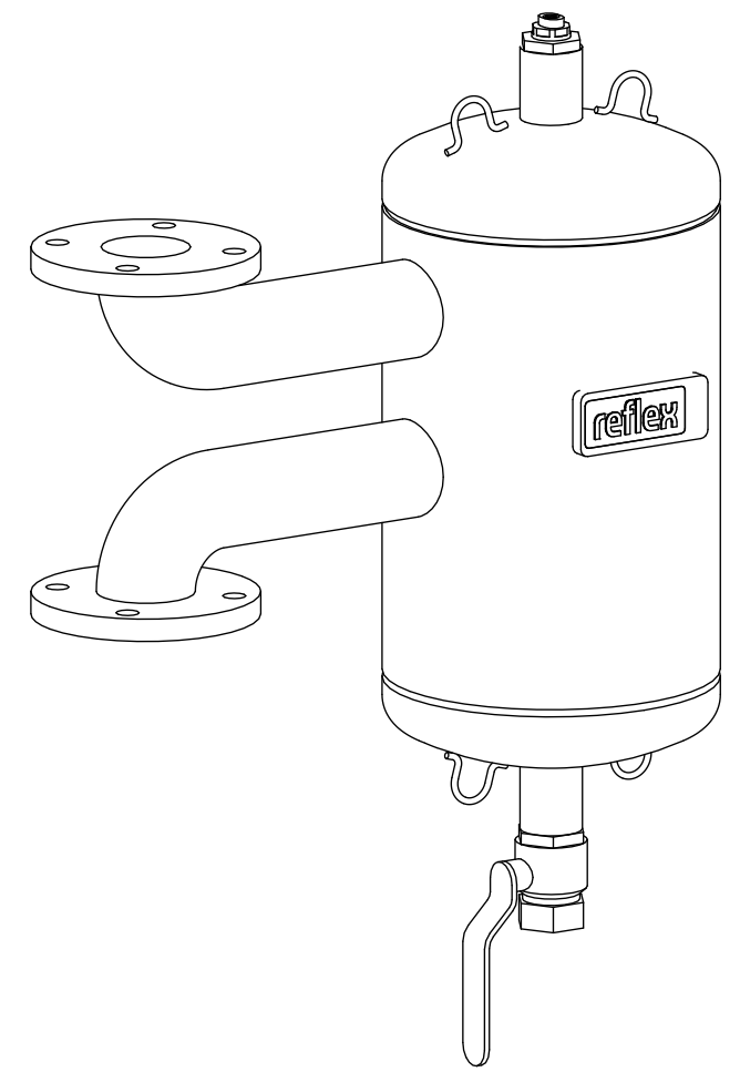
Isometric view
