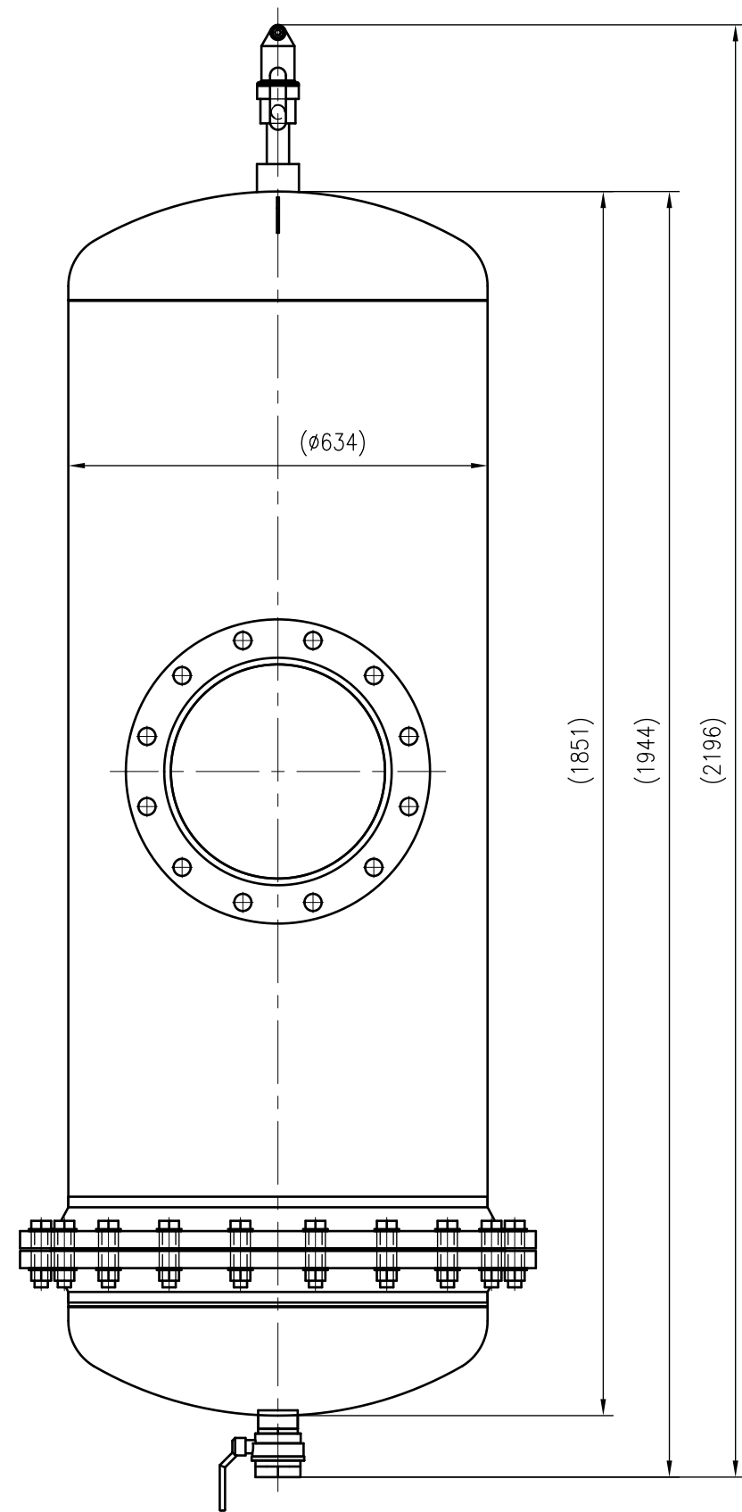
Side view
