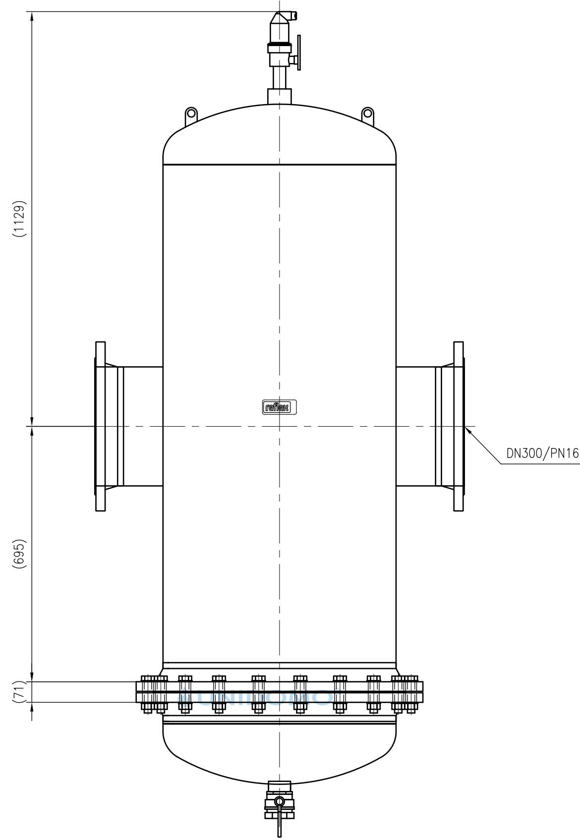
Front view
