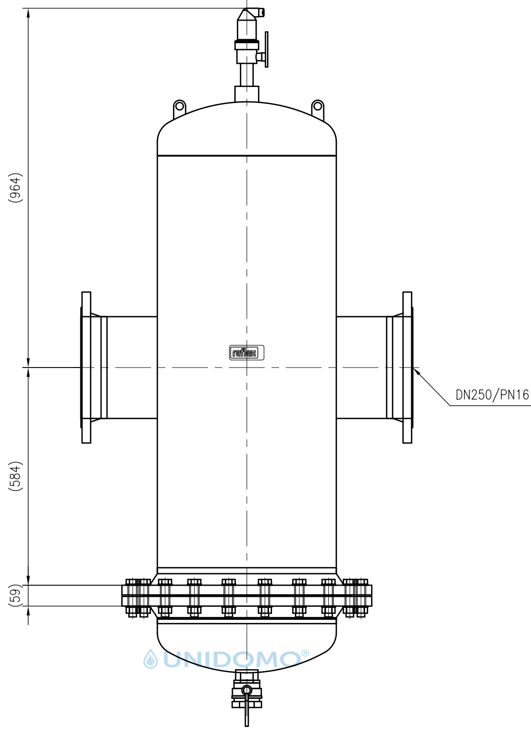
Front view
