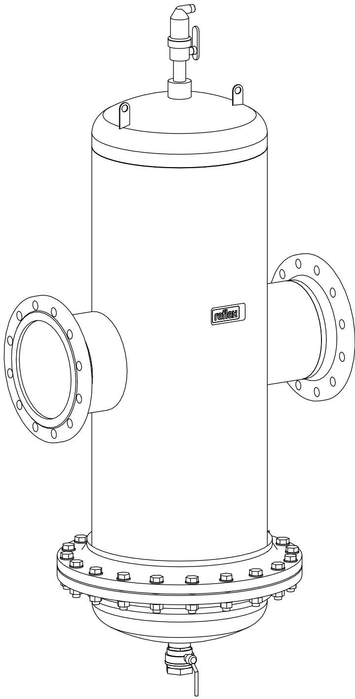
Isometric view
