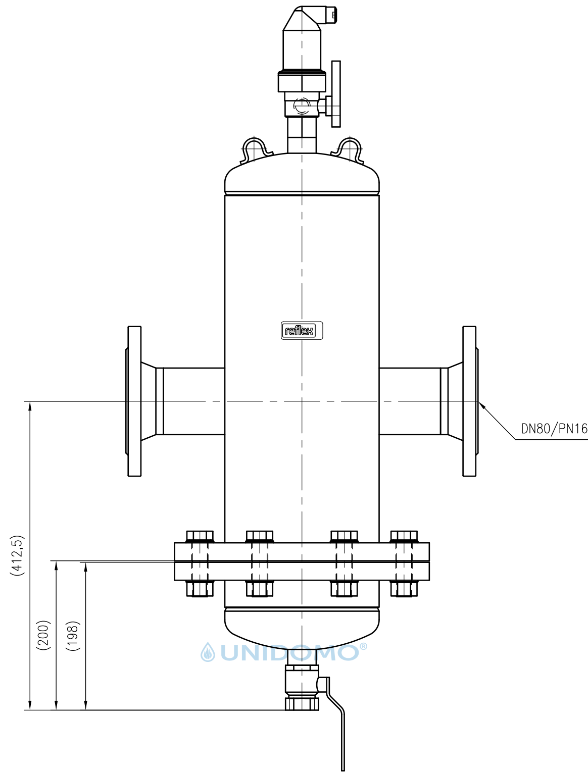
Front view
