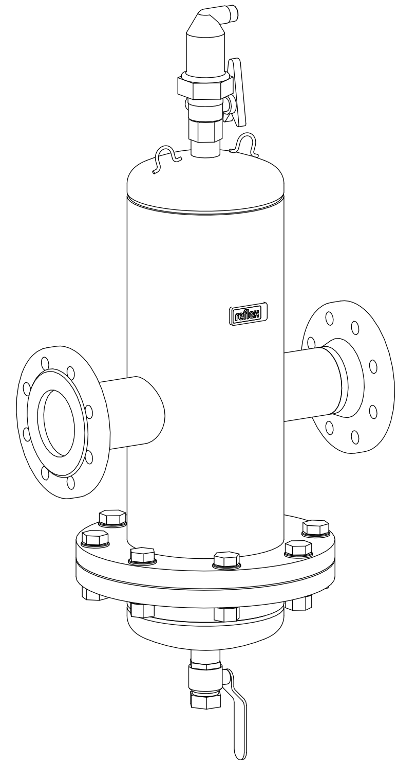
Isometric view
