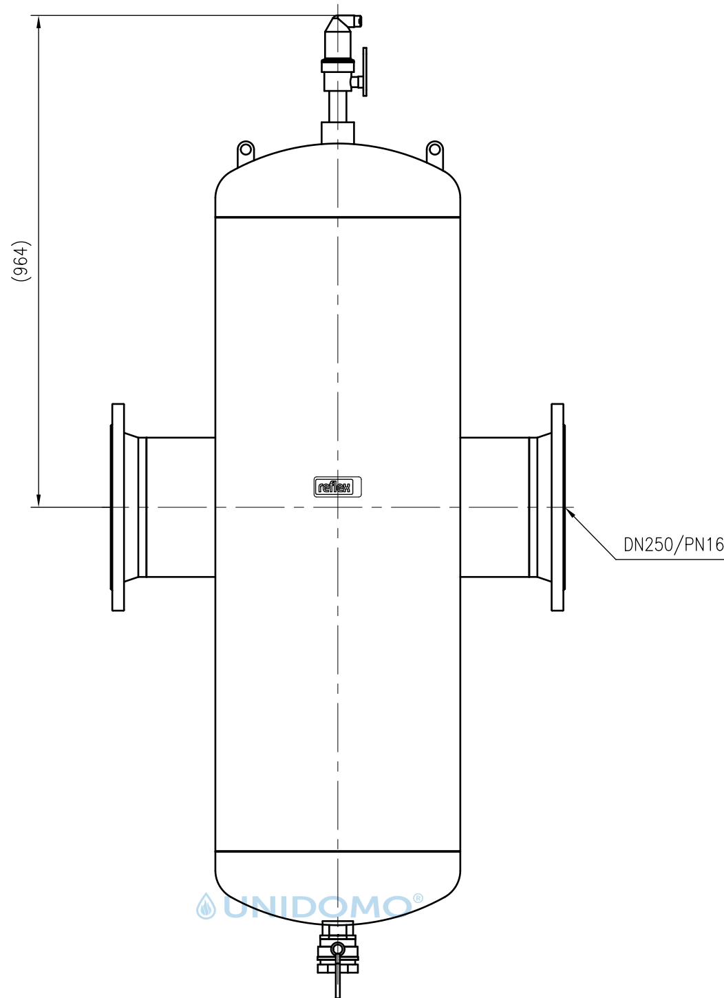
Front view
