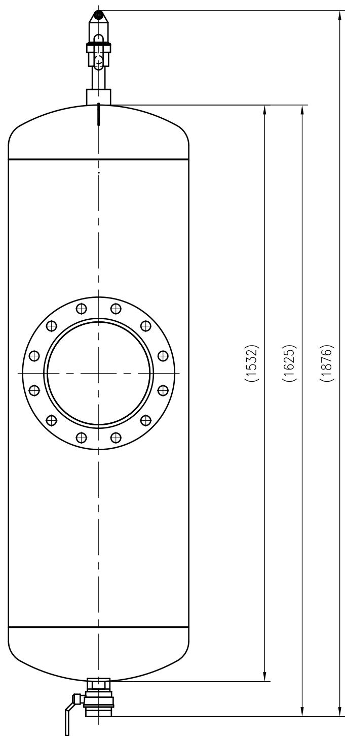
Side view
