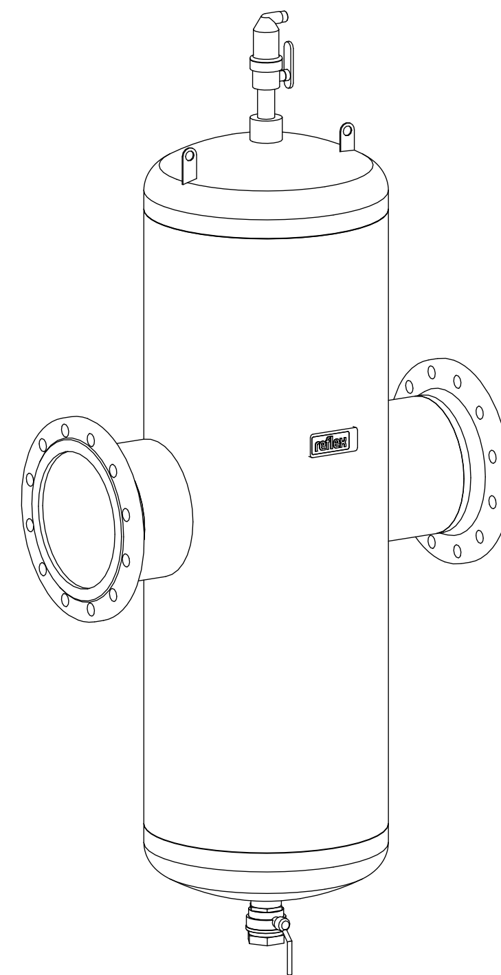
Isometric view
