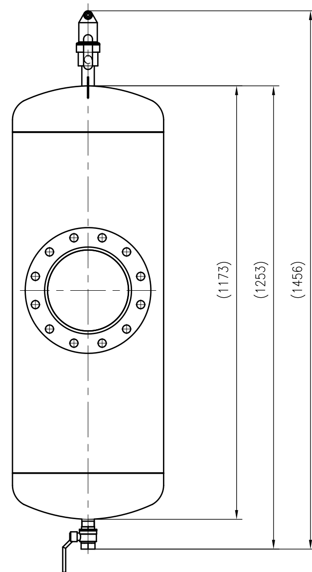
Side view
