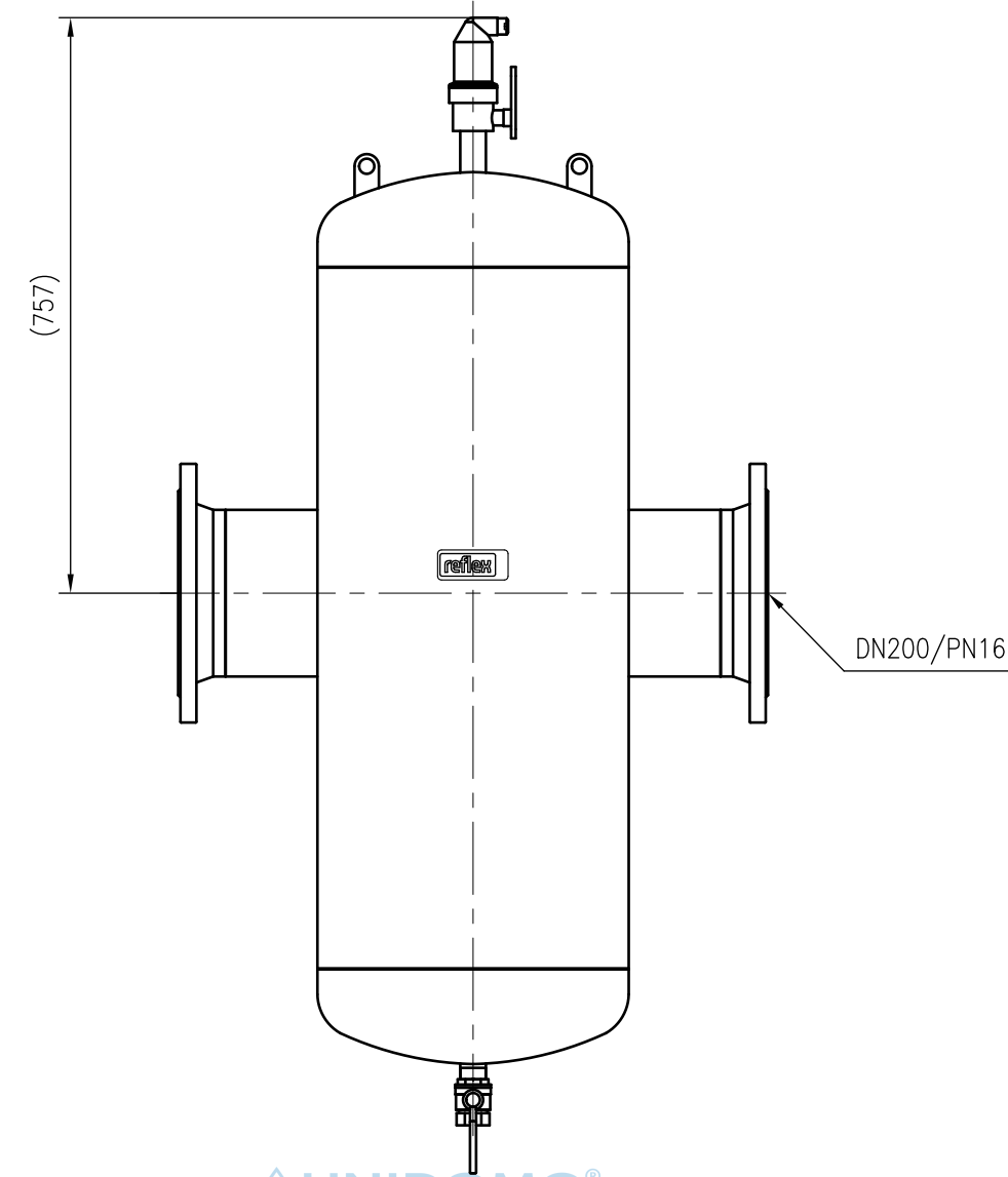
Front view
