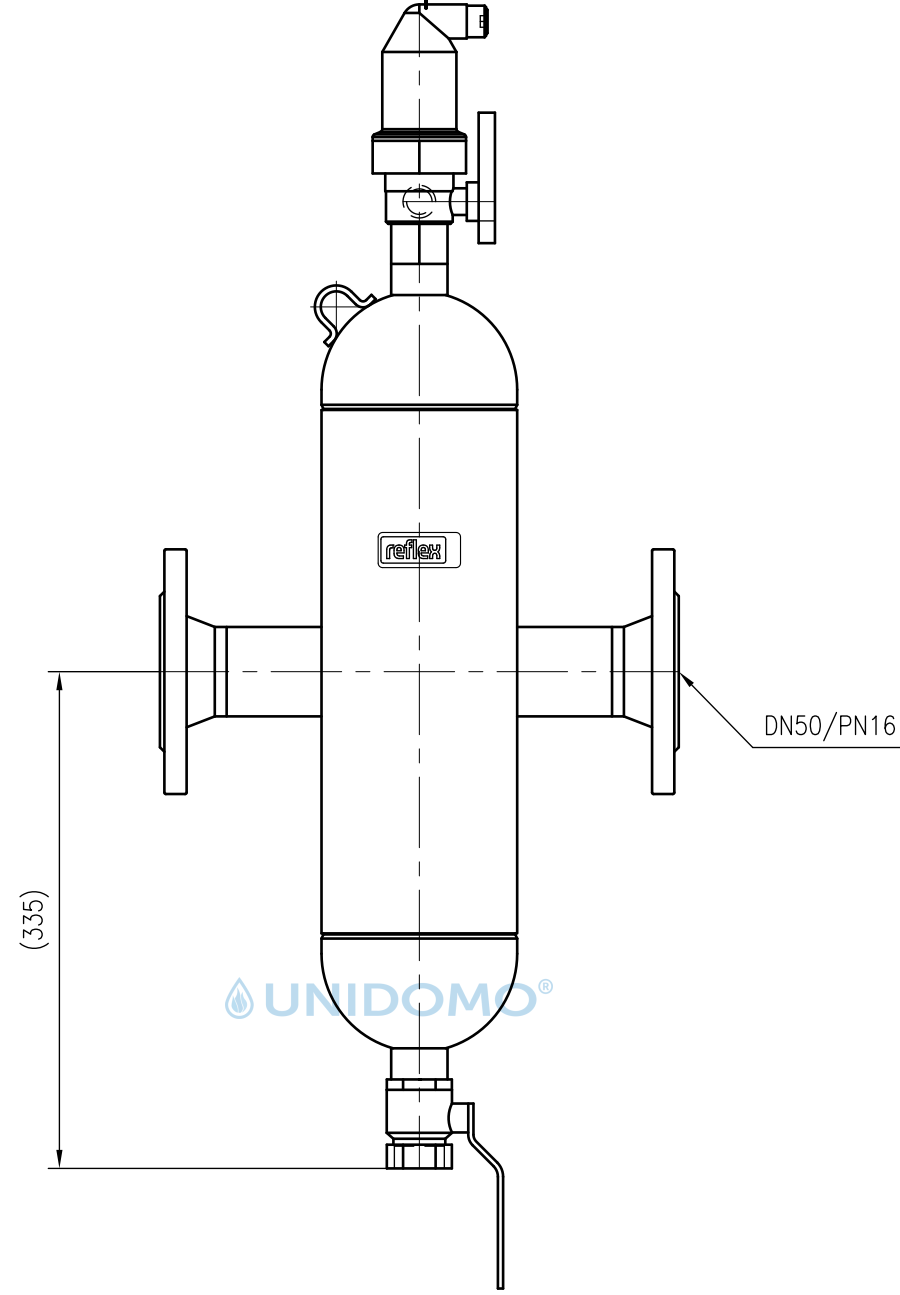
Front view
