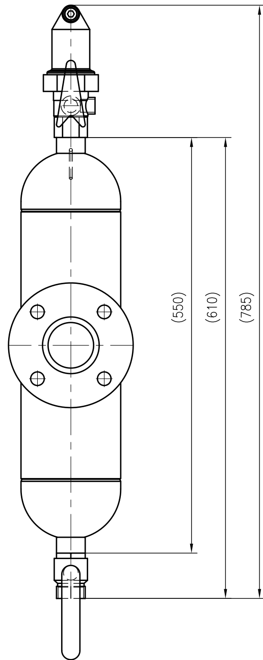
Side view
