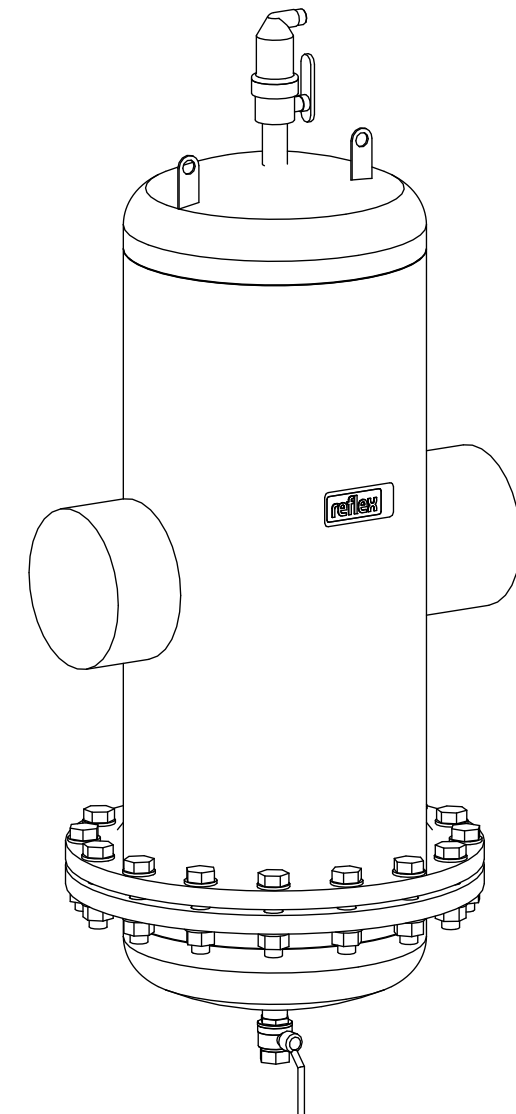
Isometric view
