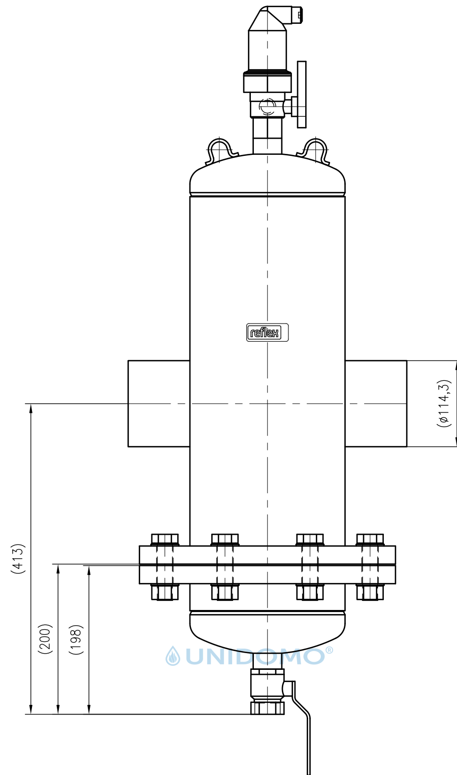
Front view
