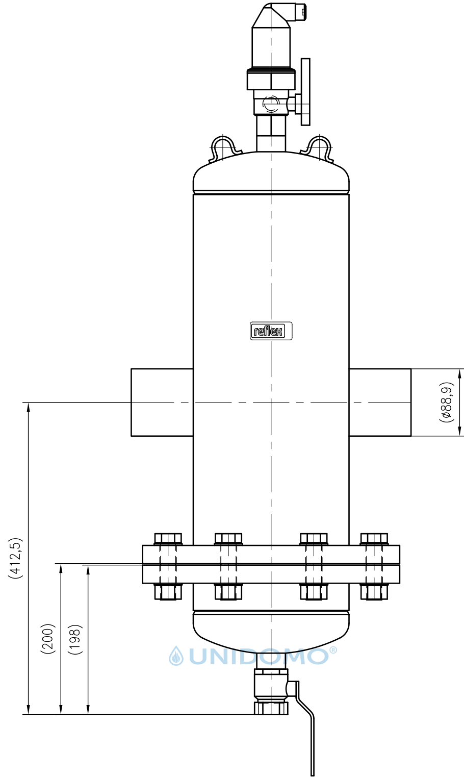
Front view
