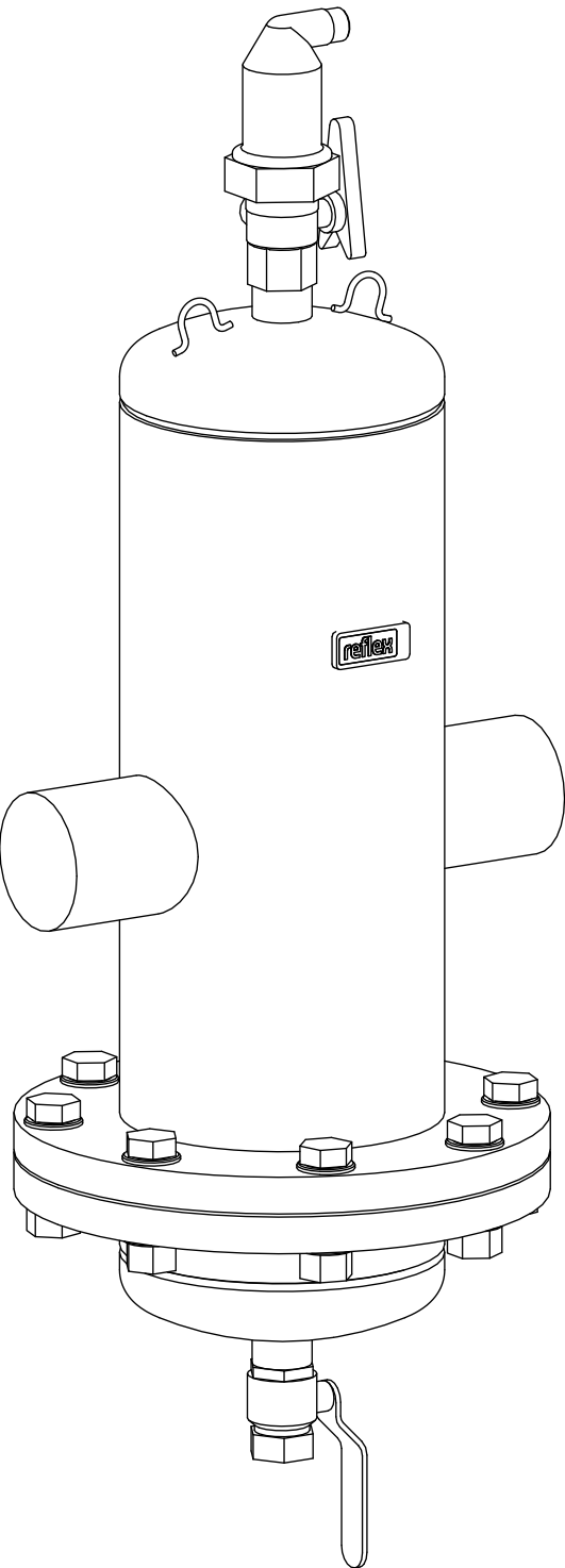
Isometric view
