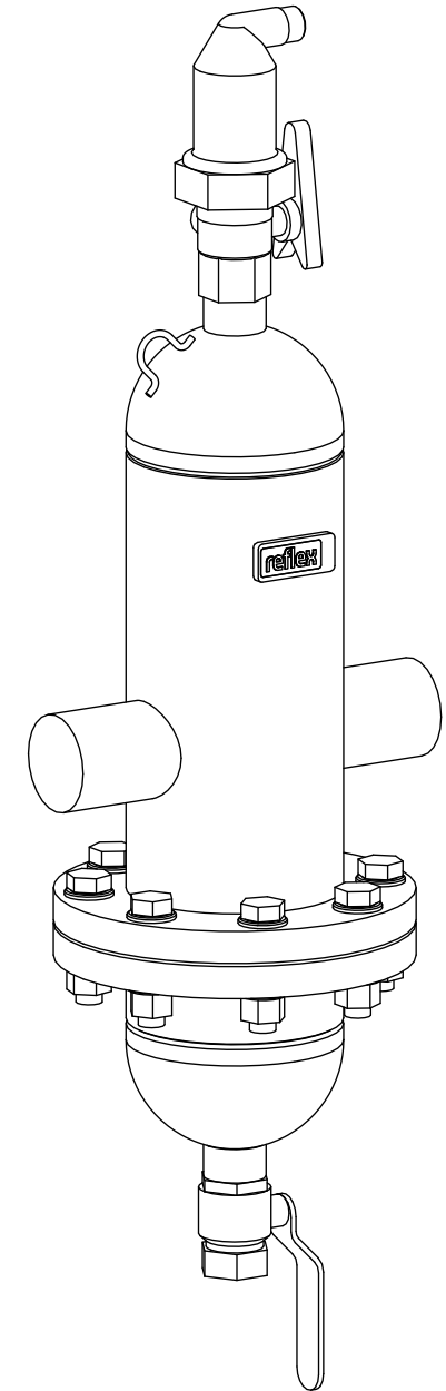
Isometric view
