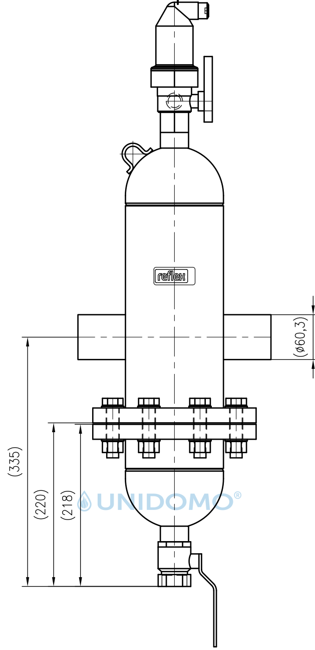
Front view
