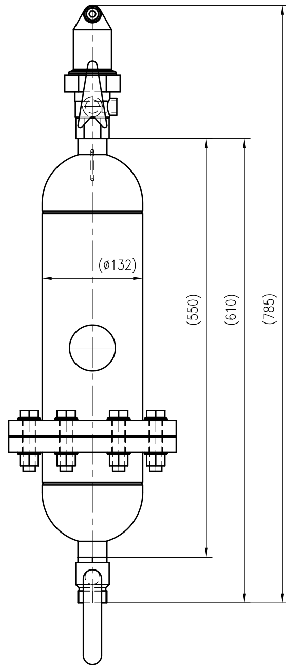
Side view
