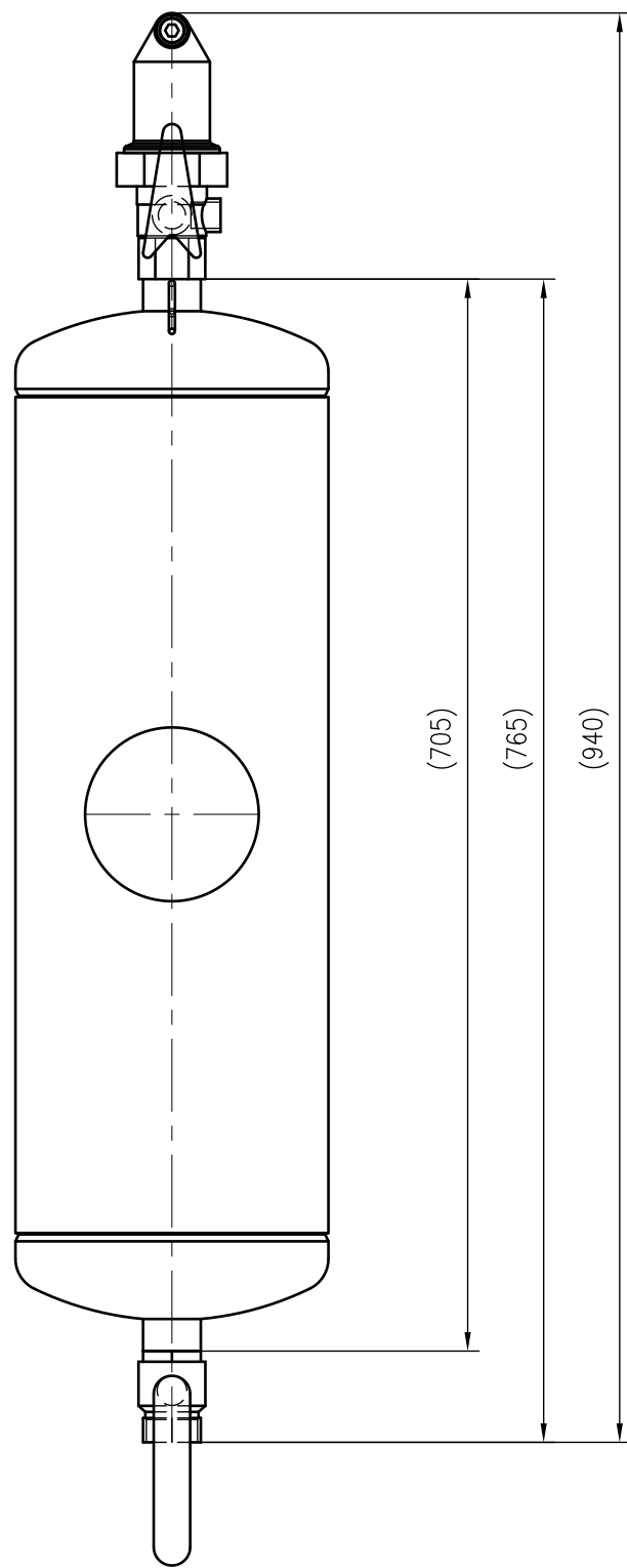
Side view
