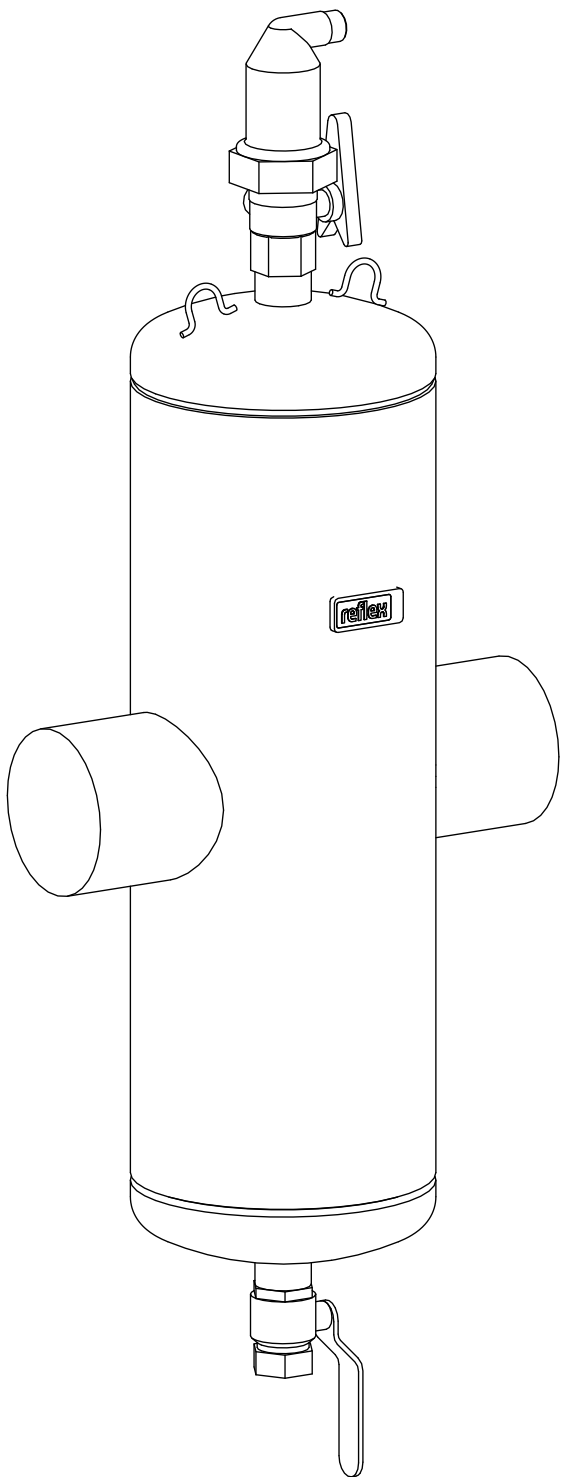
Isometric view
