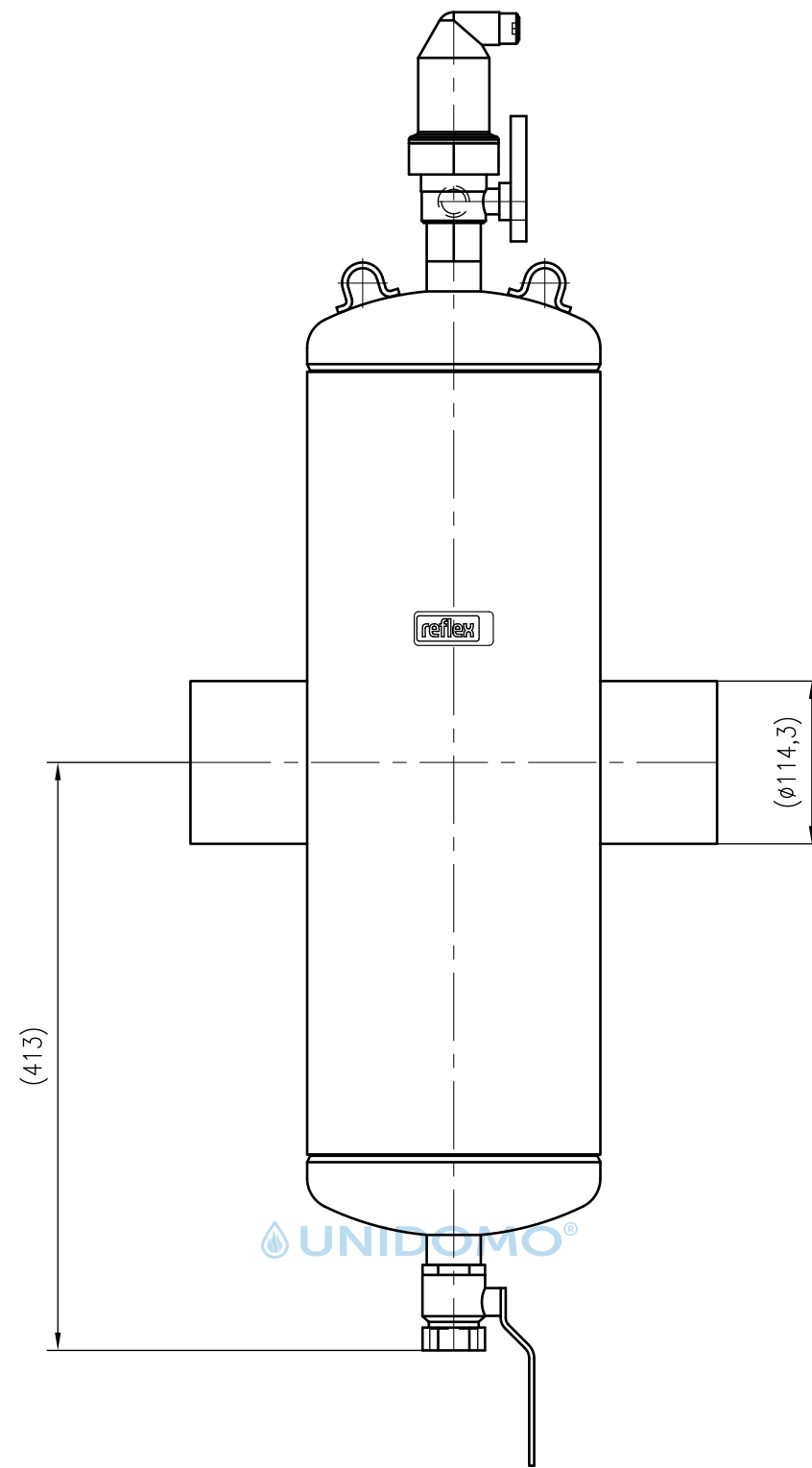
Front view
