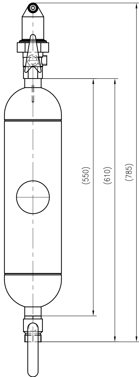
Side view
