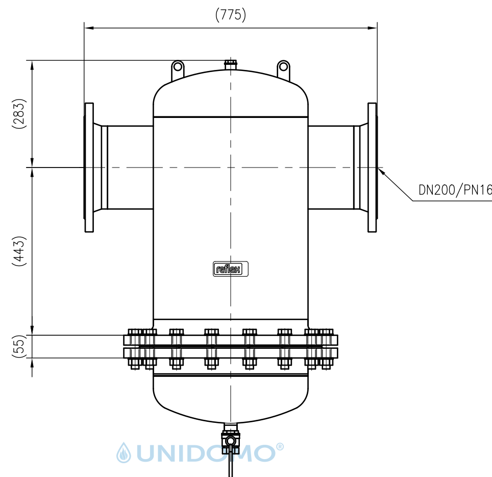
Front view
