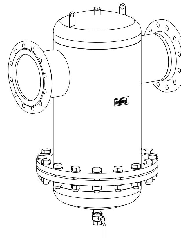
Isometric view
