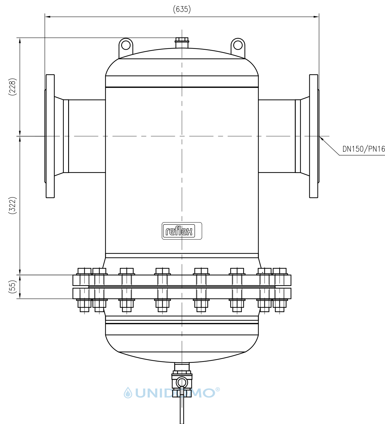
Front view
