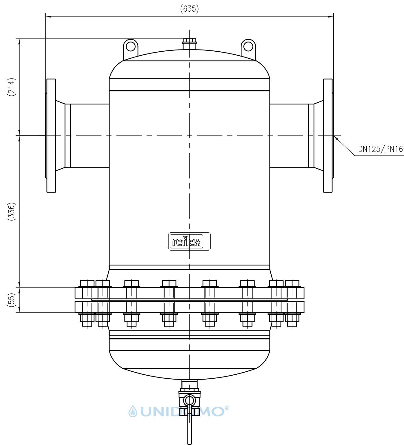
Front view
