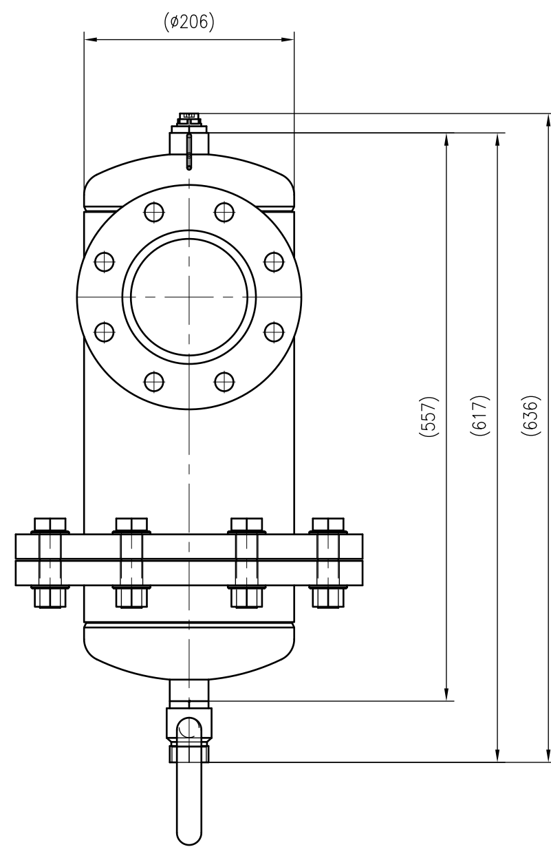
Side view
