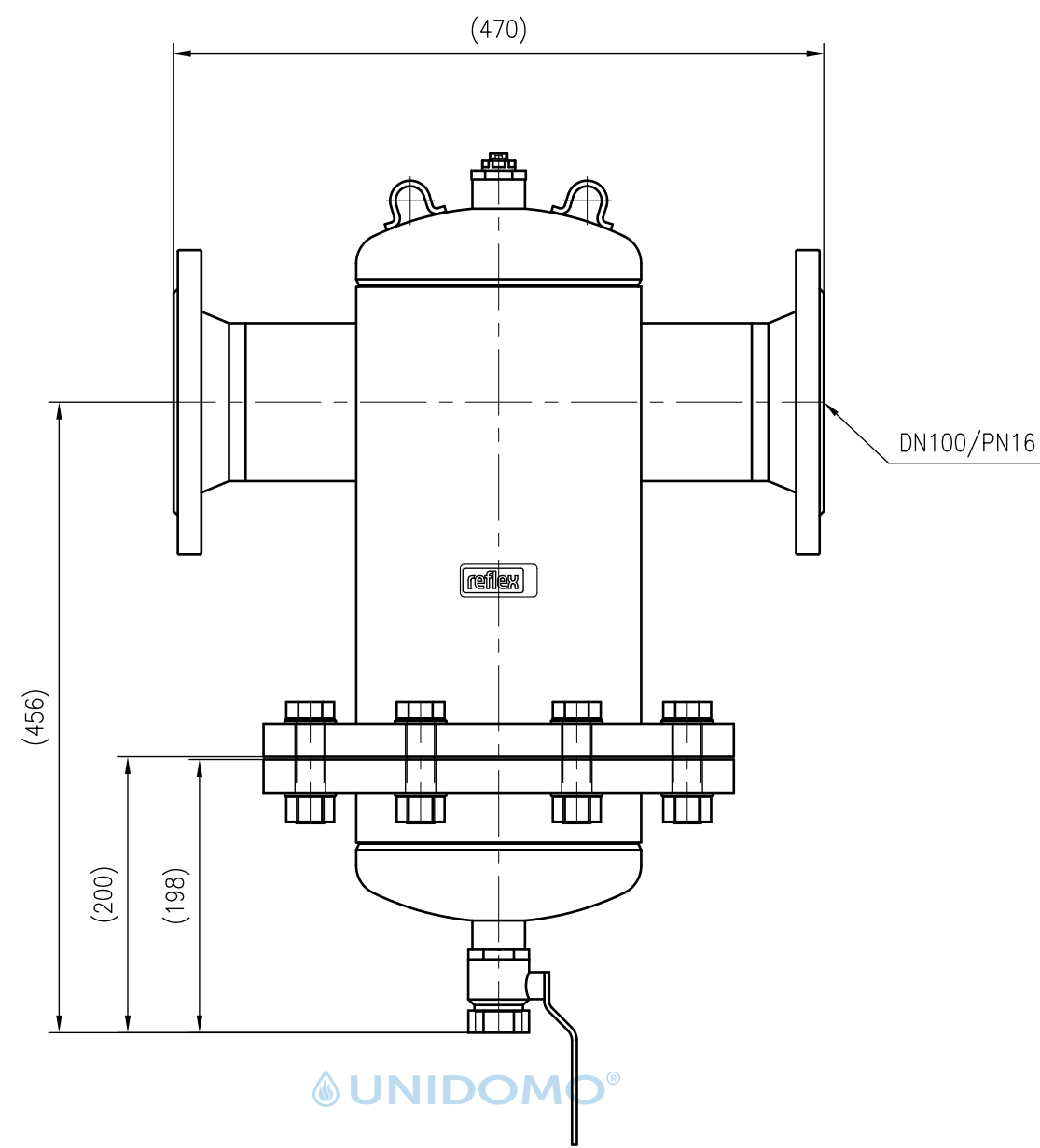
Front view
