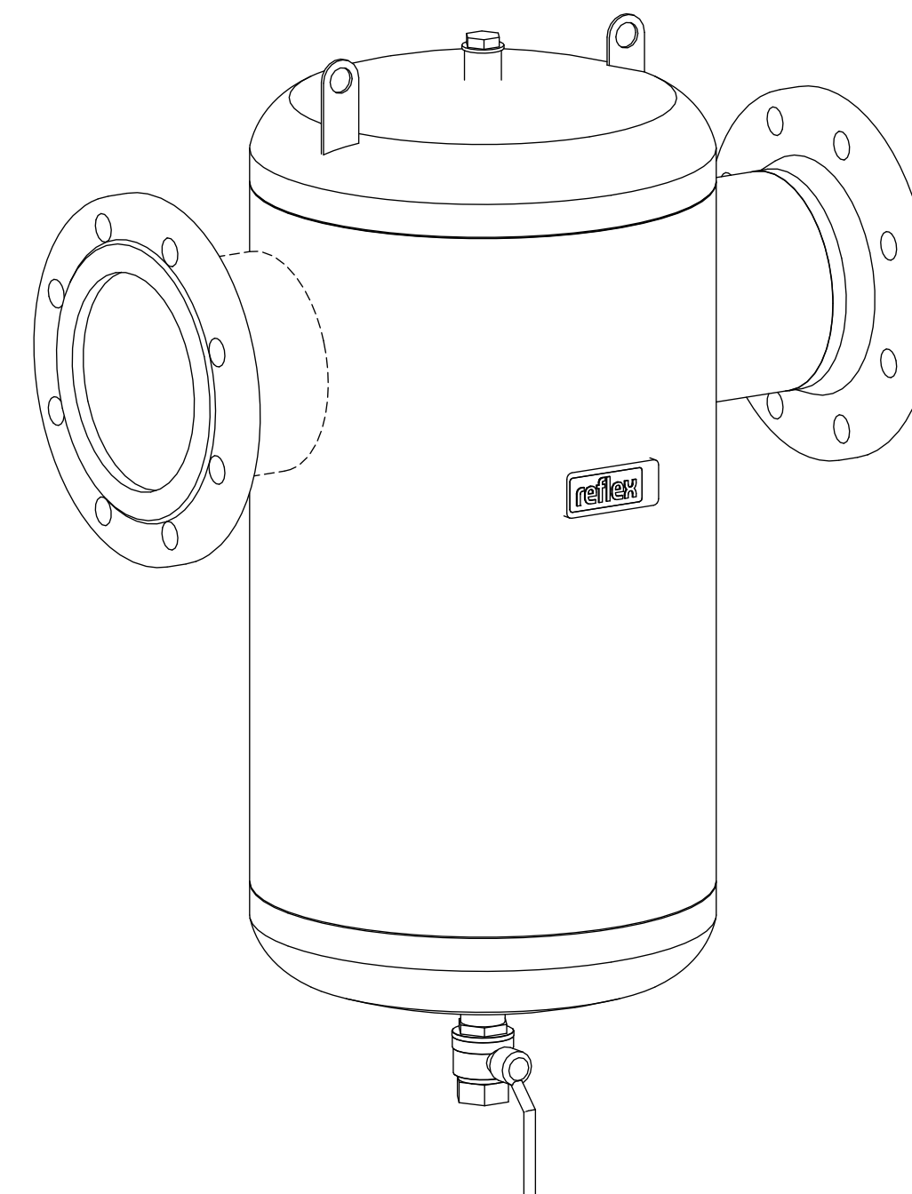
Isometric view
