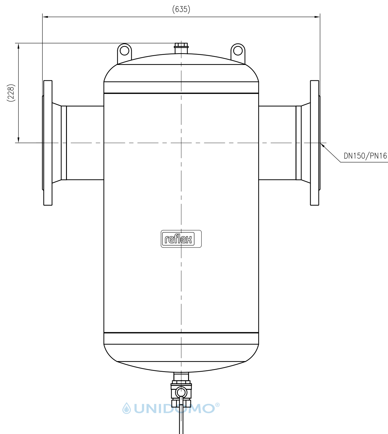
Front view
