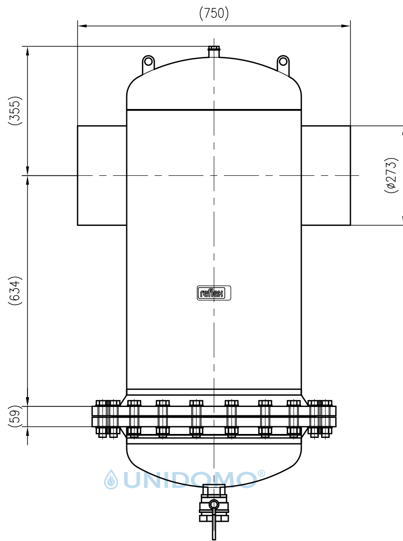
Front view
