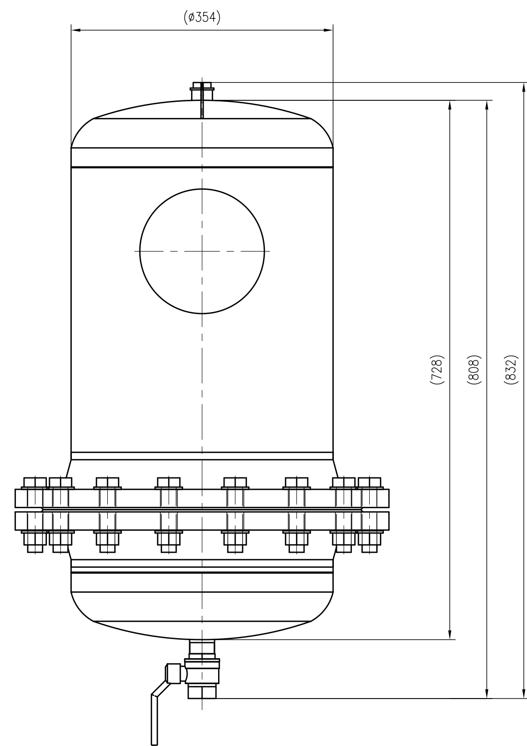
Side view
