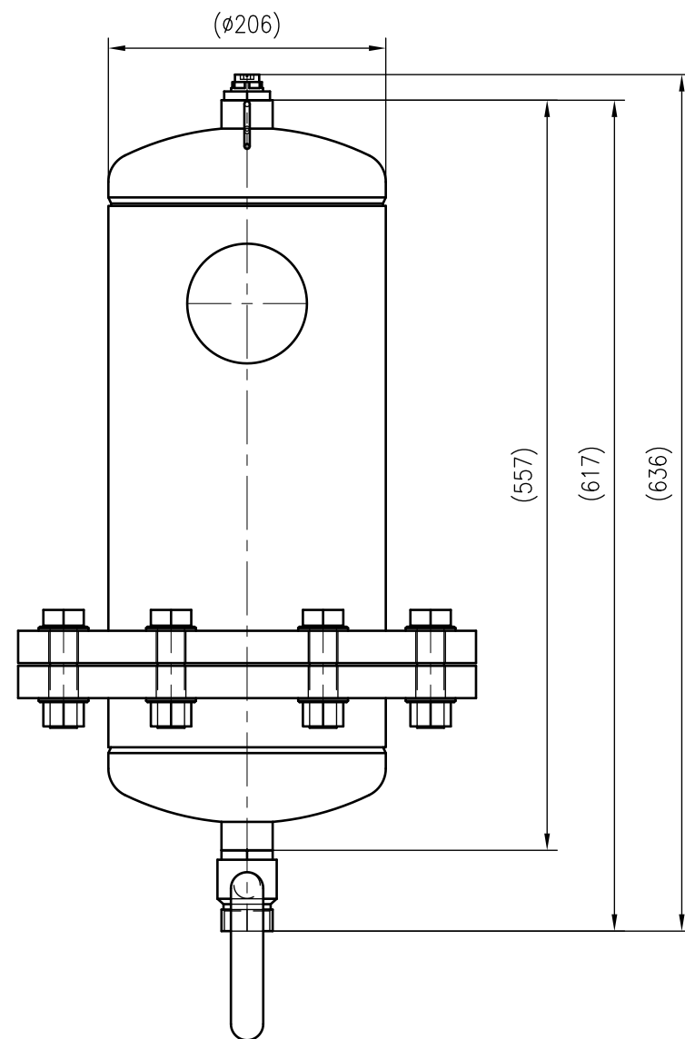
Side view
