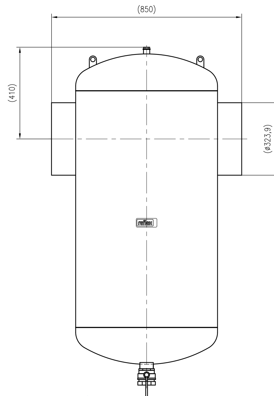
Front view
