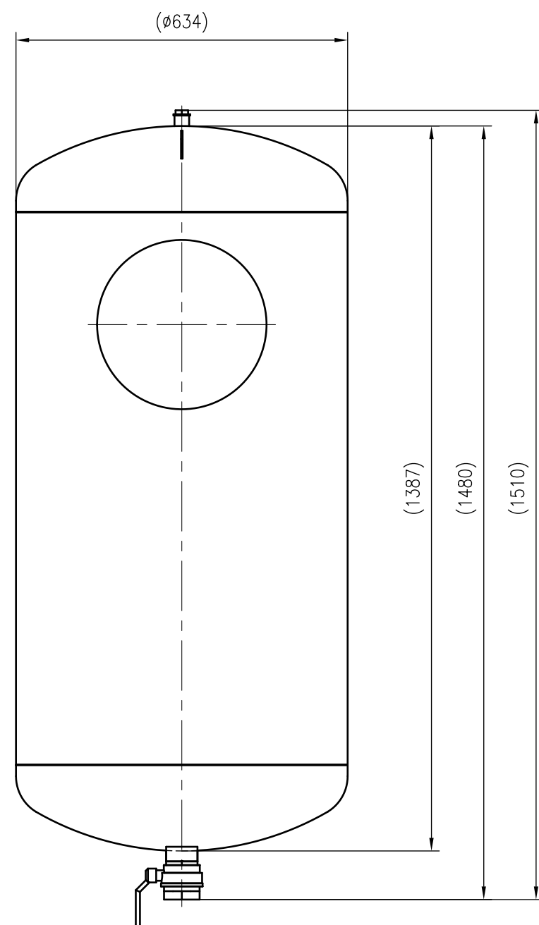
Side view
