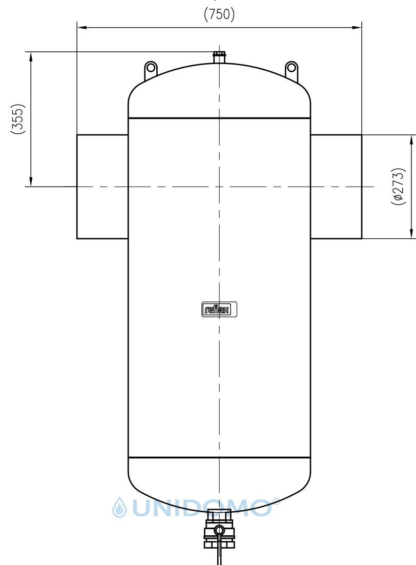
Front view
