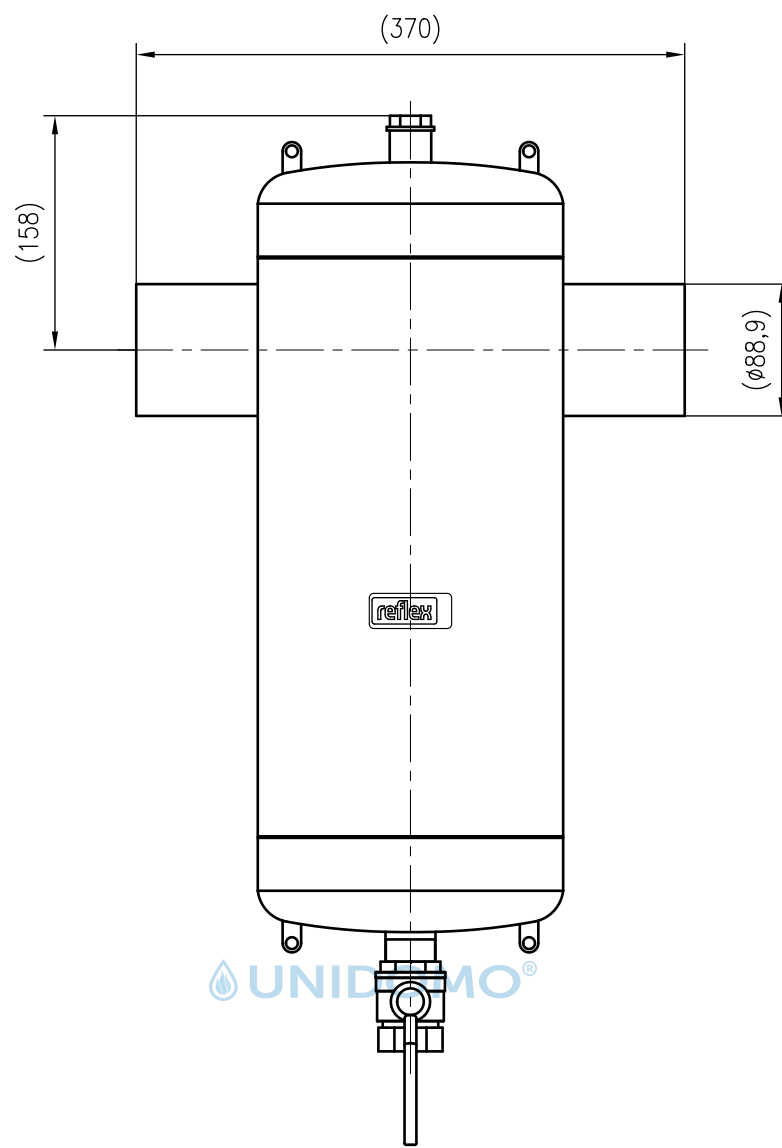
Front view
