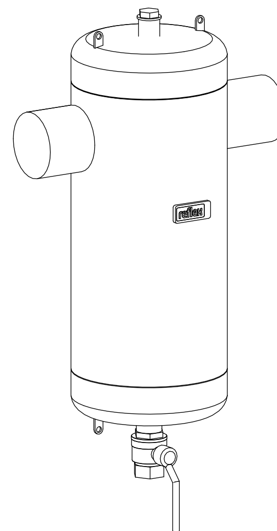
Isometric view
