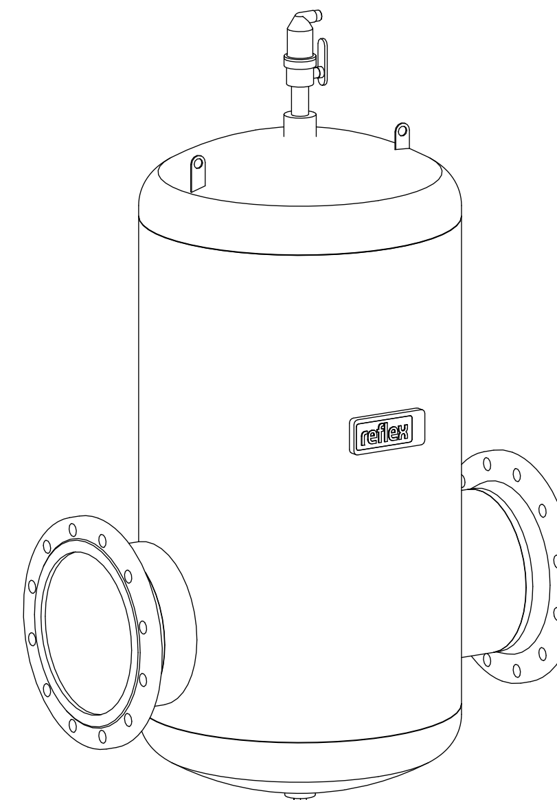
Isometric view
