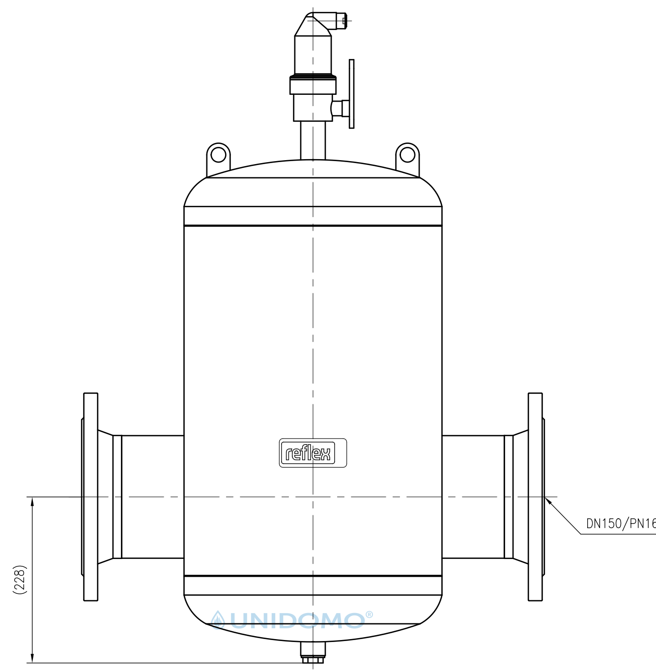
Front view
