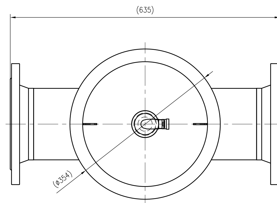
Top view
