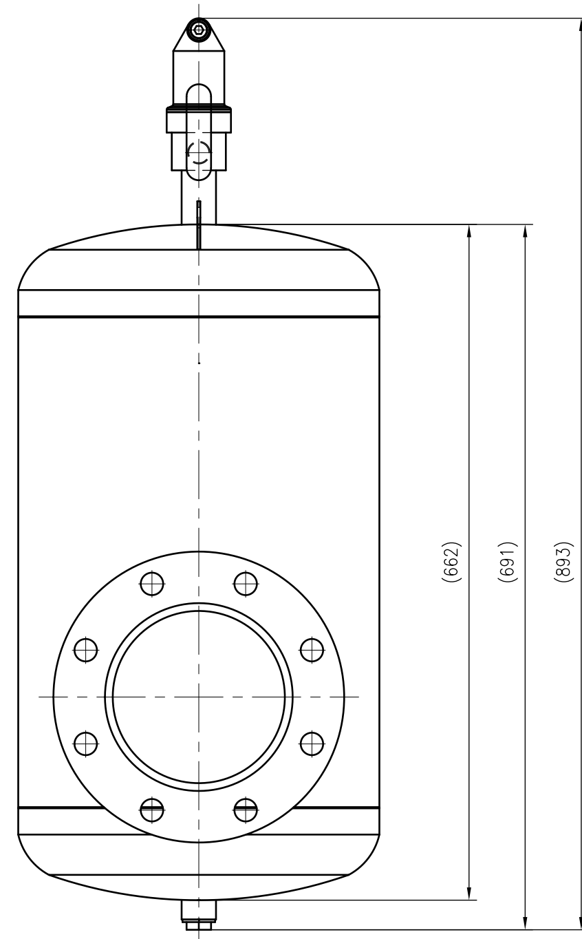
Side view
