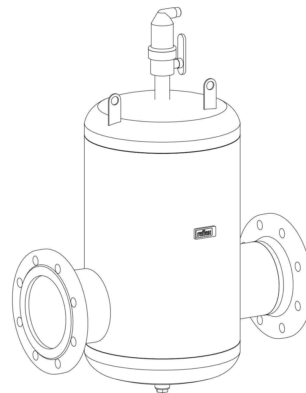
Isometric view
