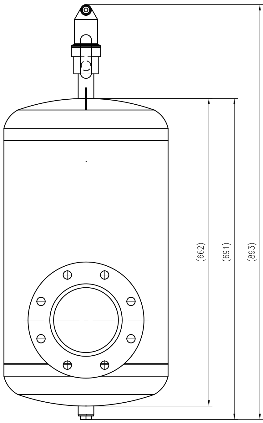
Side view
