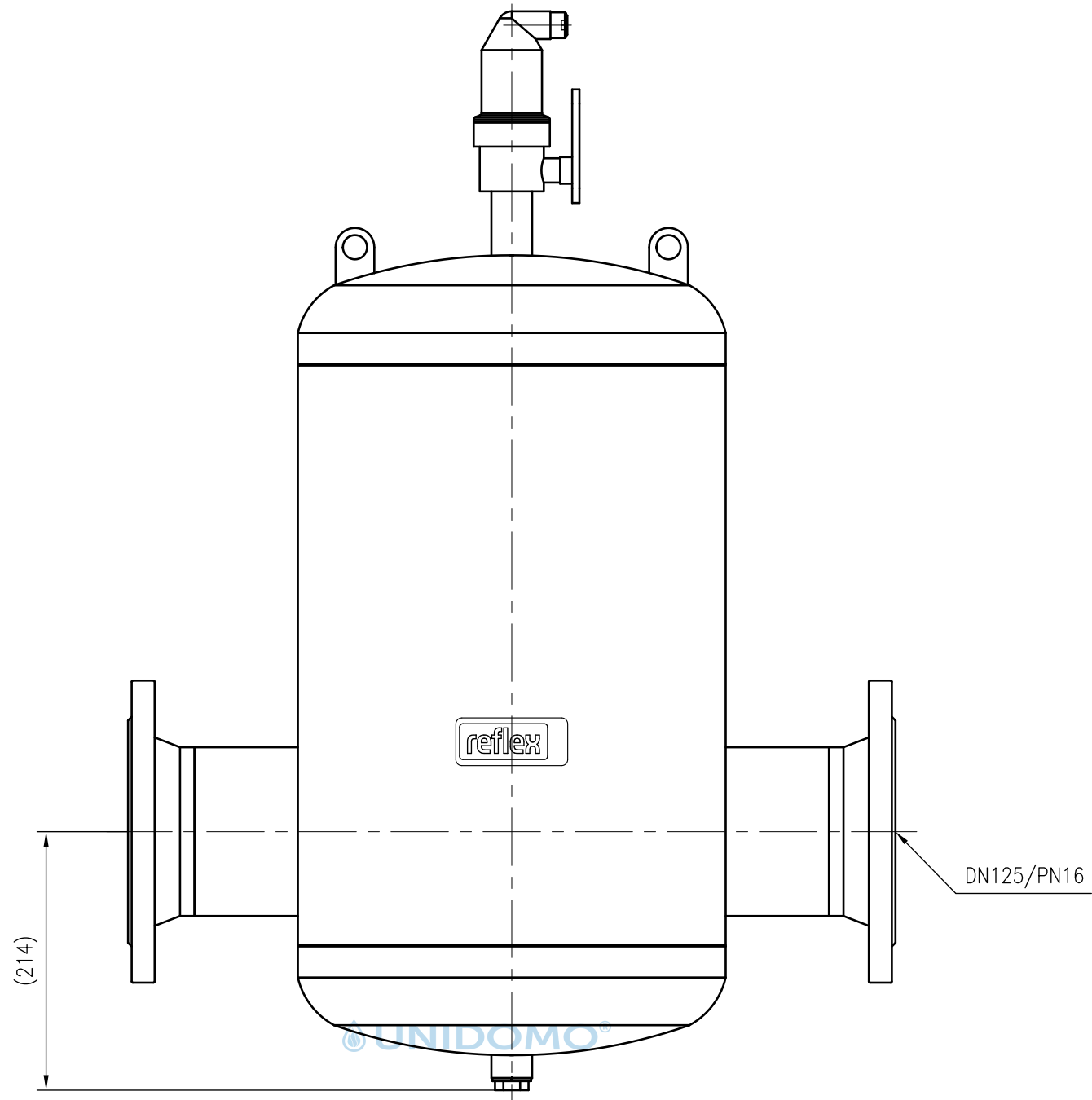
Front view
