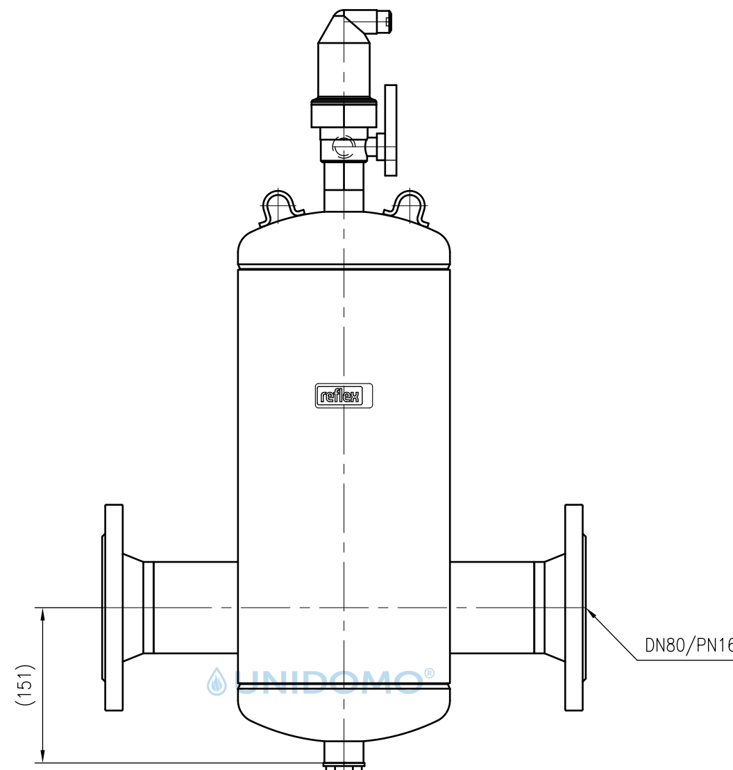
Front view
