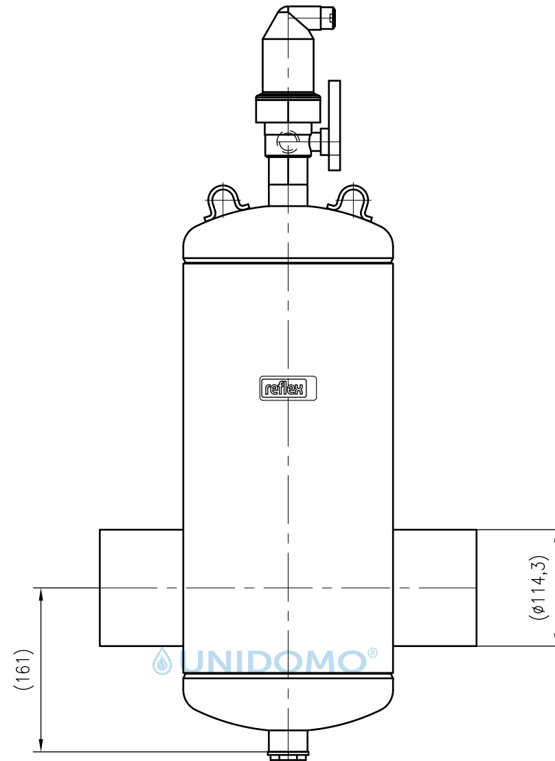
Front view
