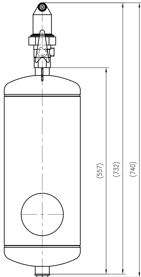
Side view
