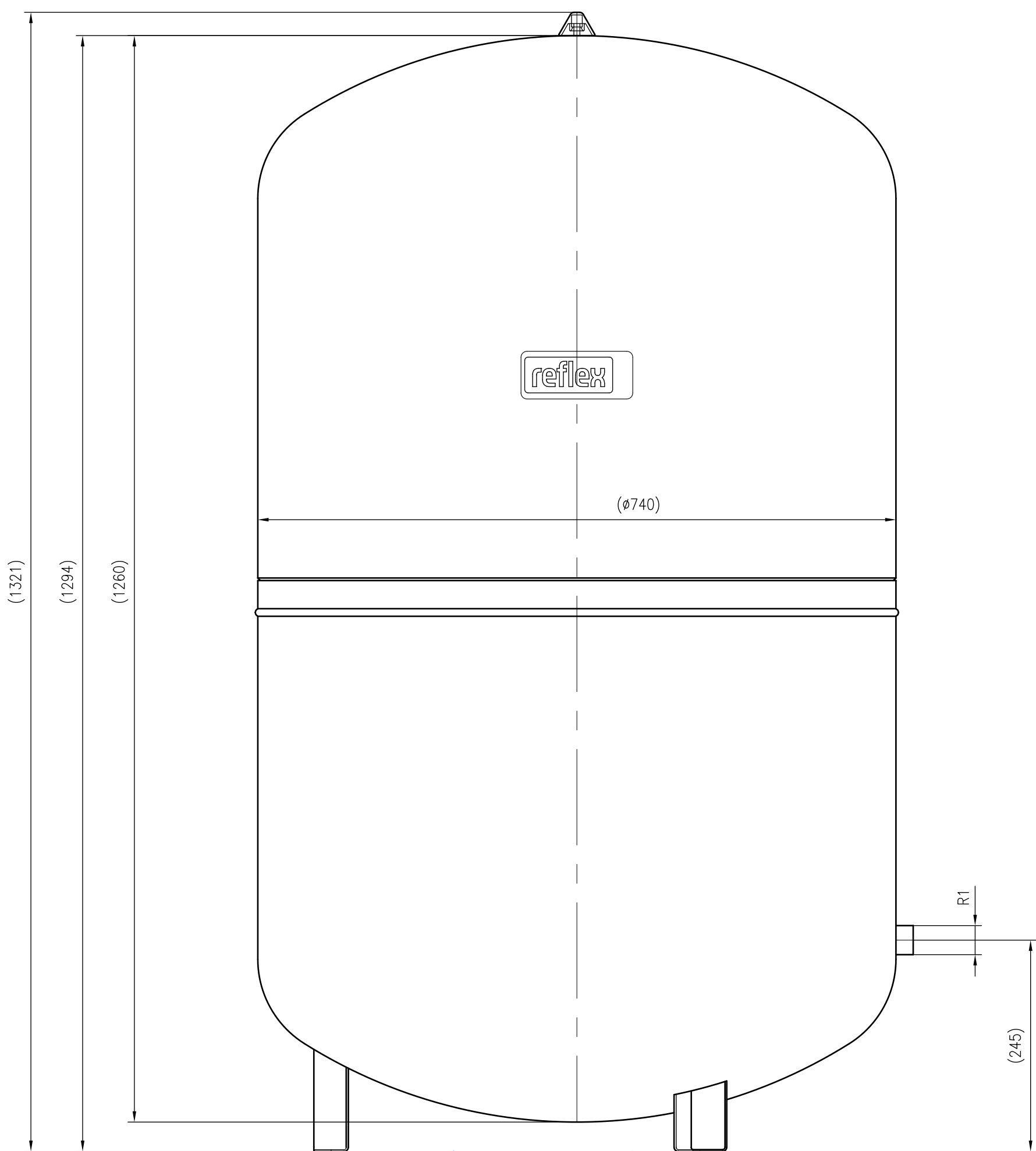
Front view
