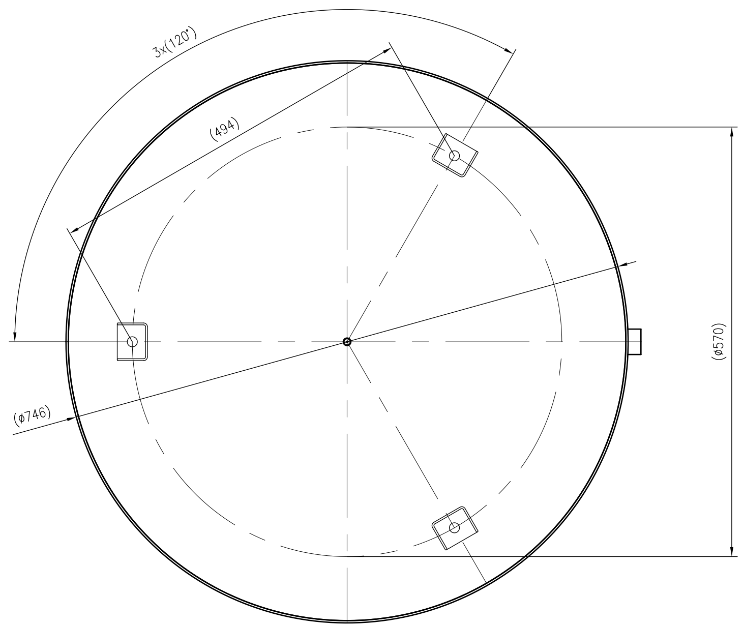
Top view
