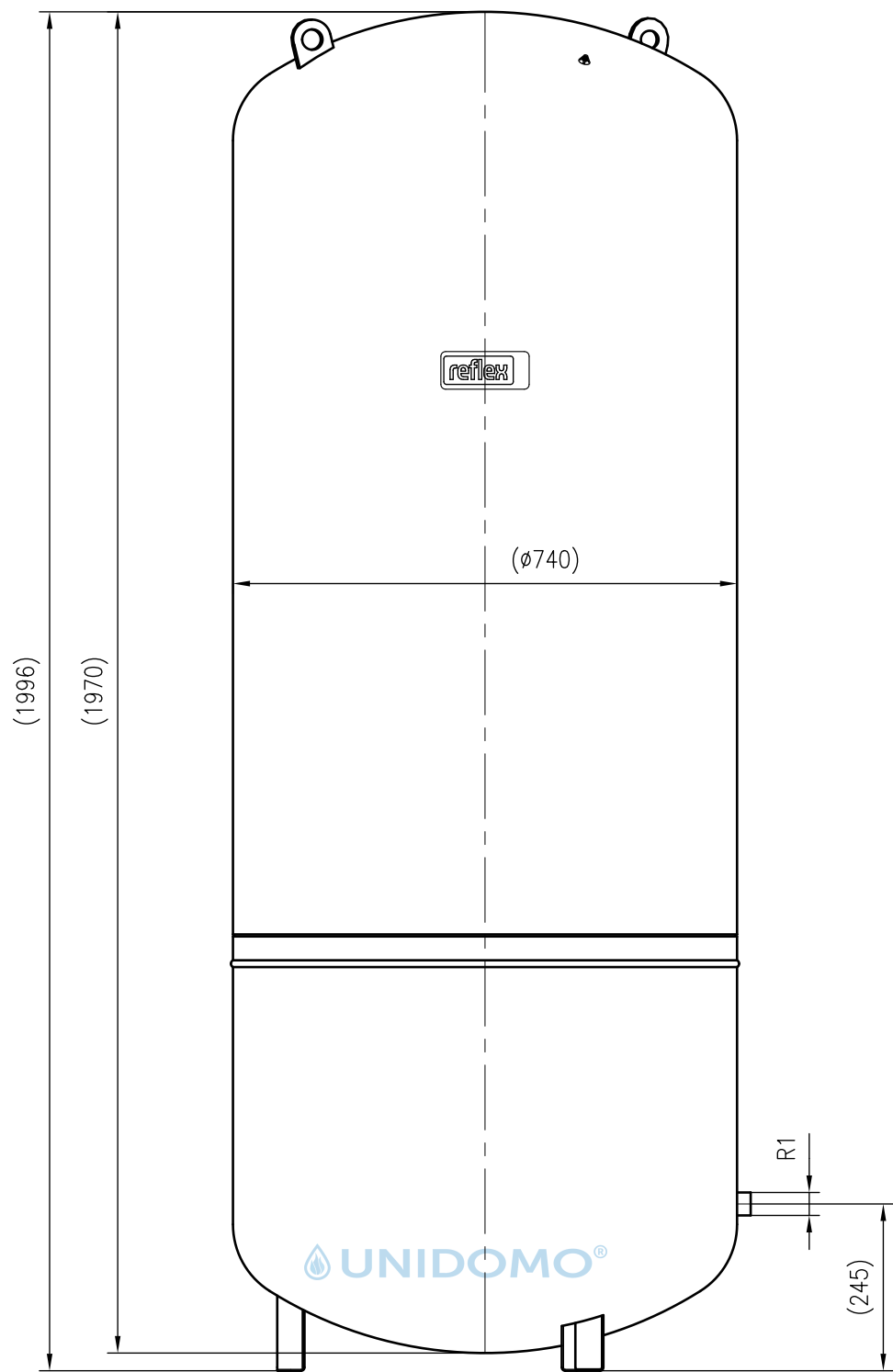
Front view
