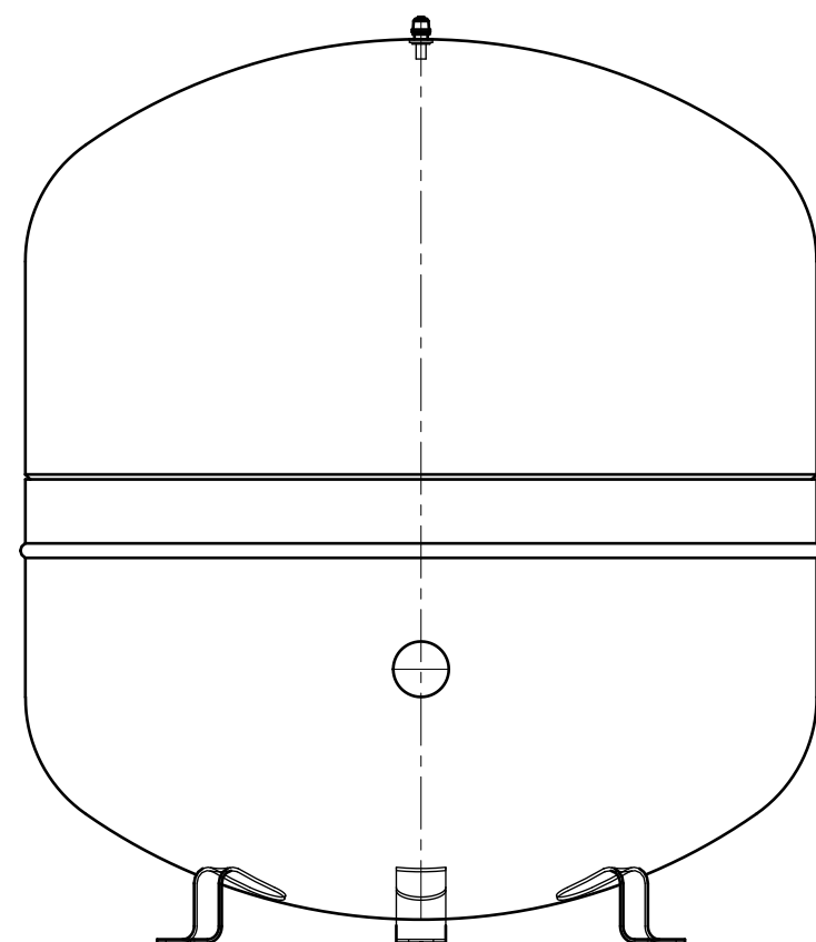
Side view
