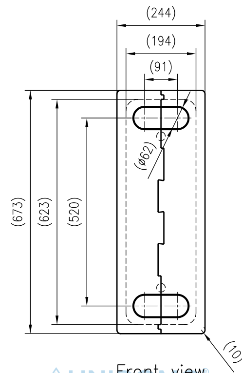
Front view
