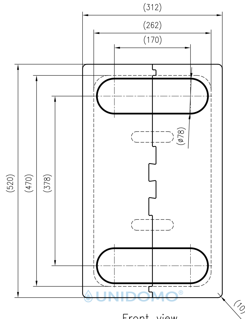
Front view
