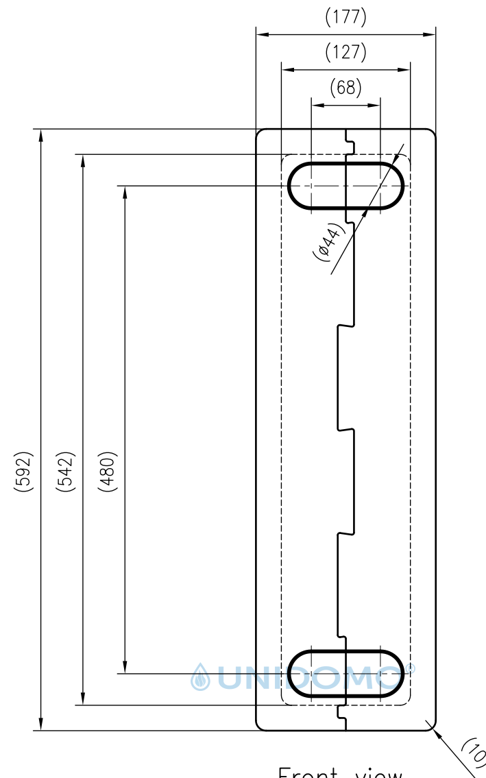
Front view
