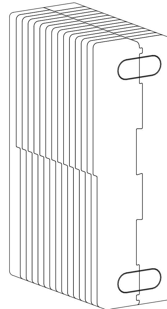
Isometric view
