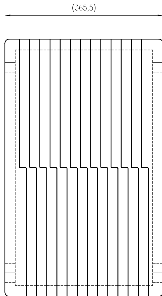
Side view
