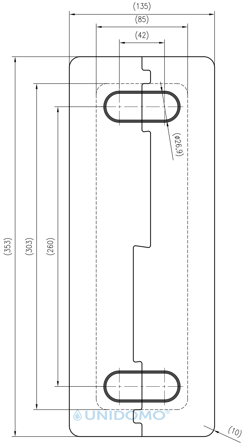
Front view
