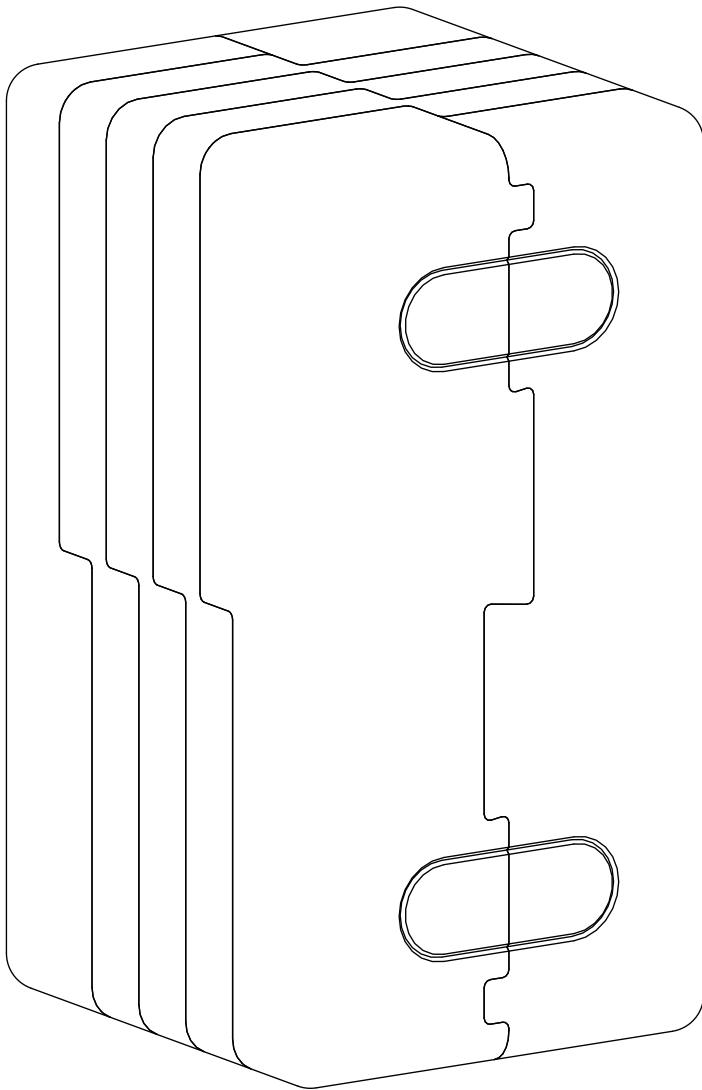
Isometric view
