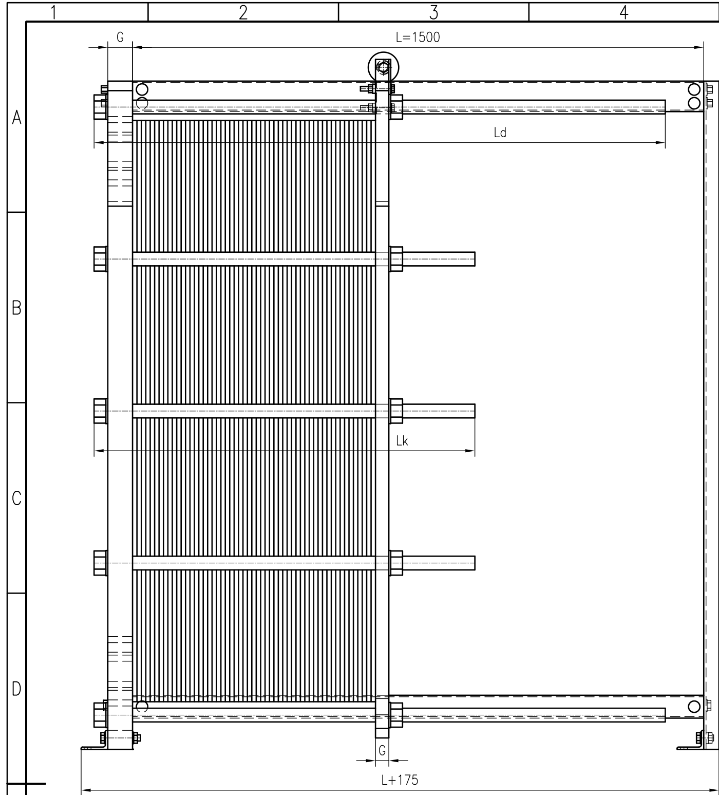
Side view
