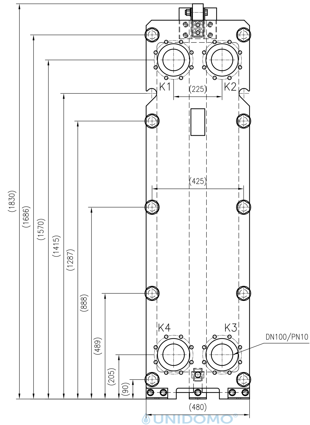
Front view
