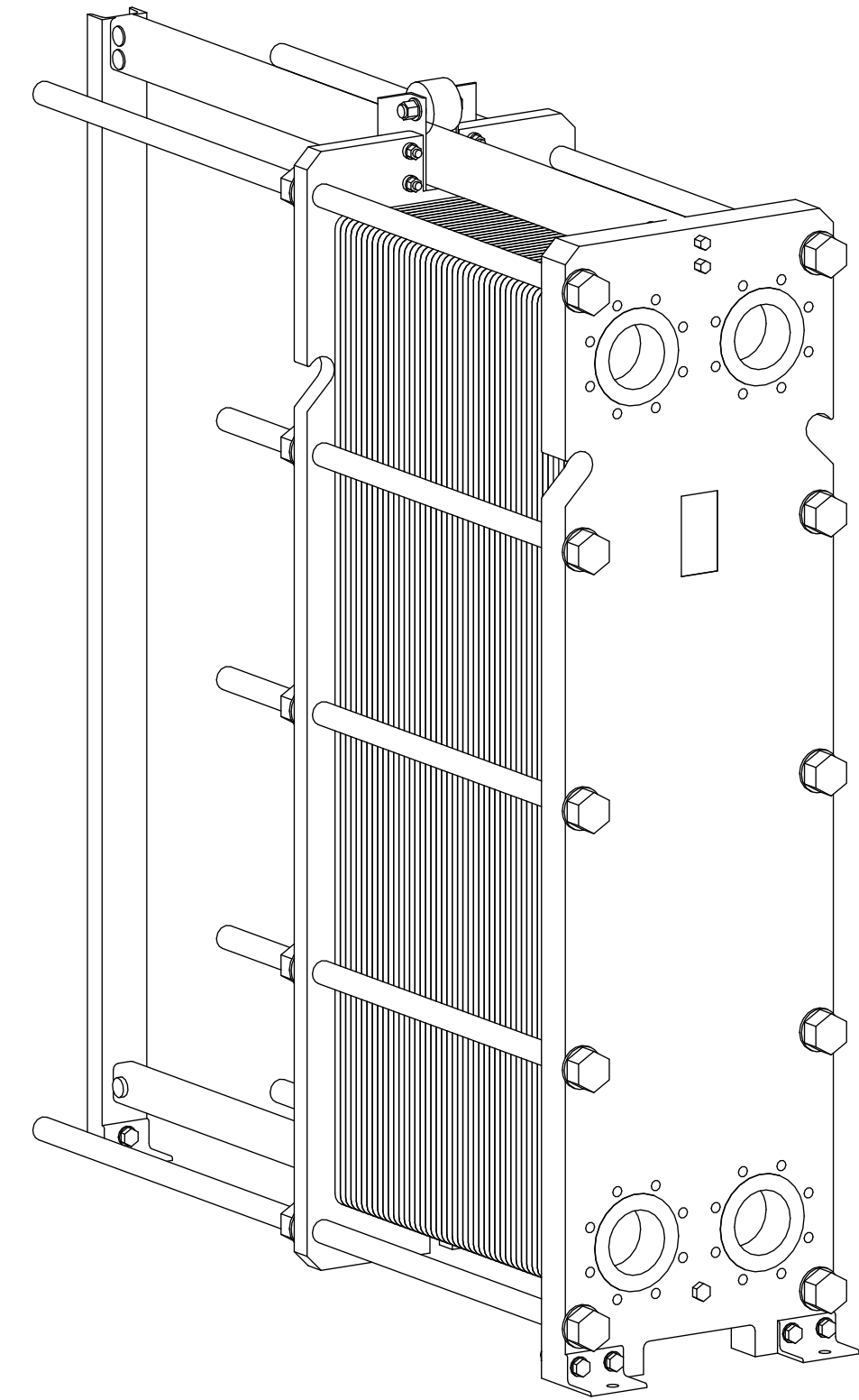
Isometric view
