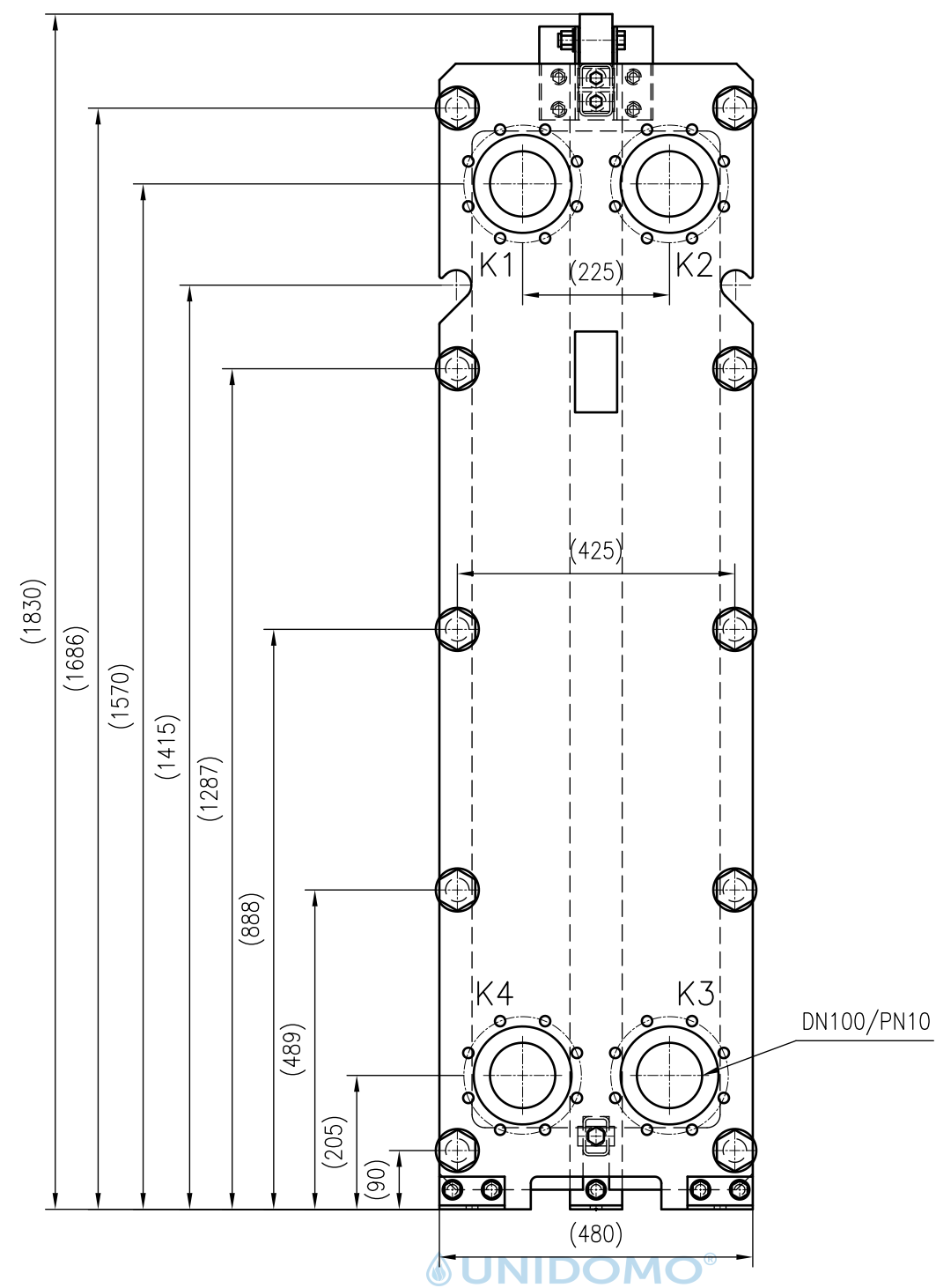
Front view
