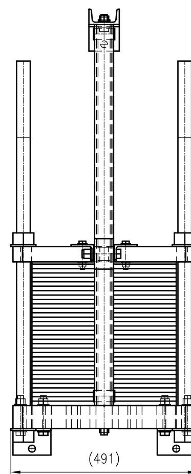
Top view
