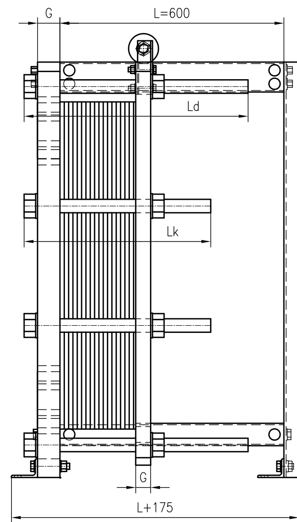
Side view
