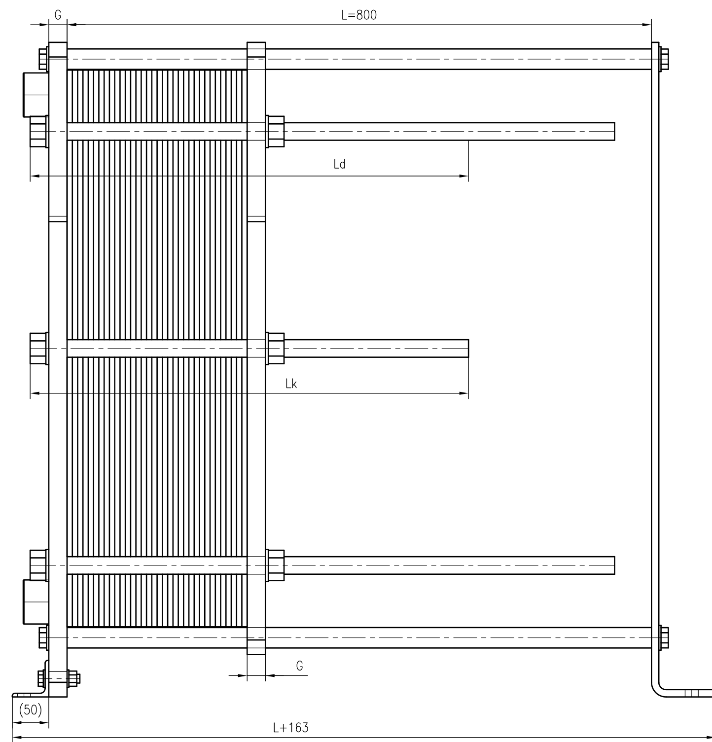
Side view
