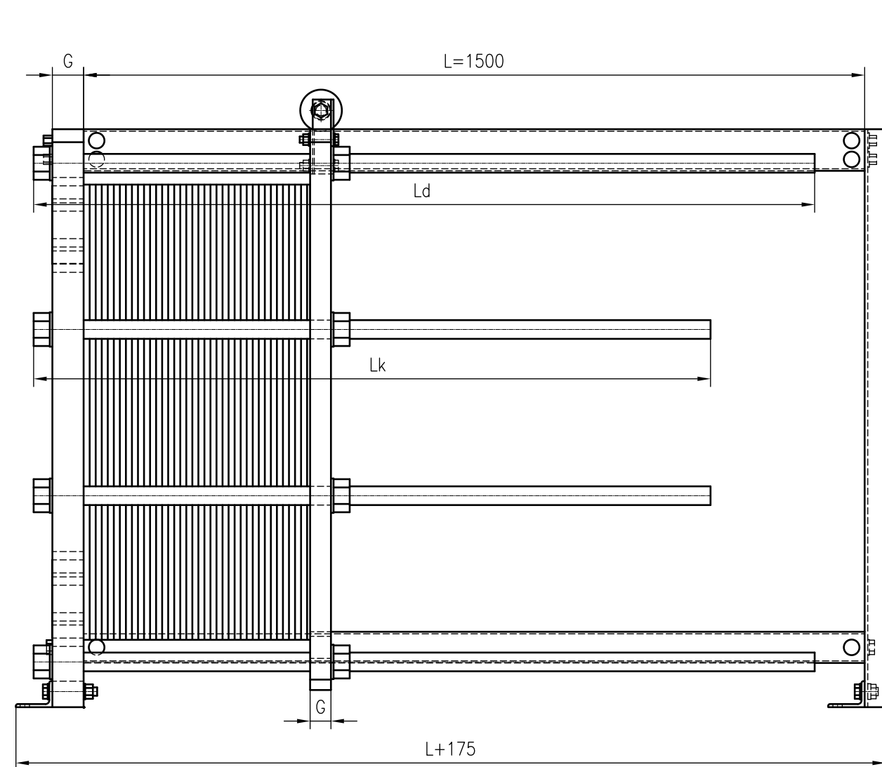
Side view
