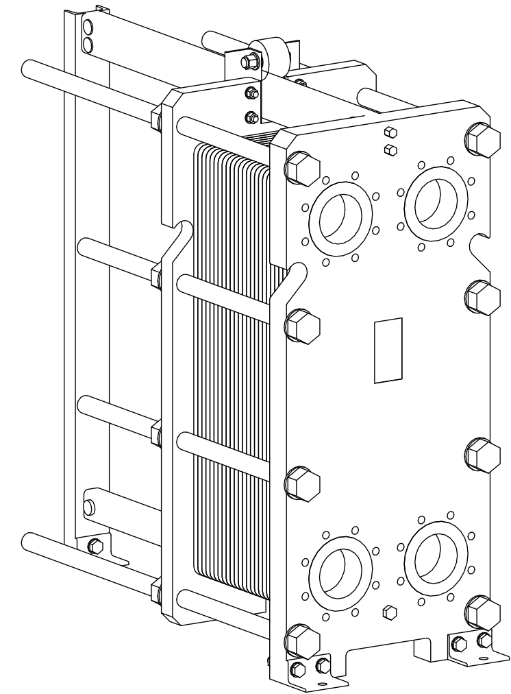
Isometric view
