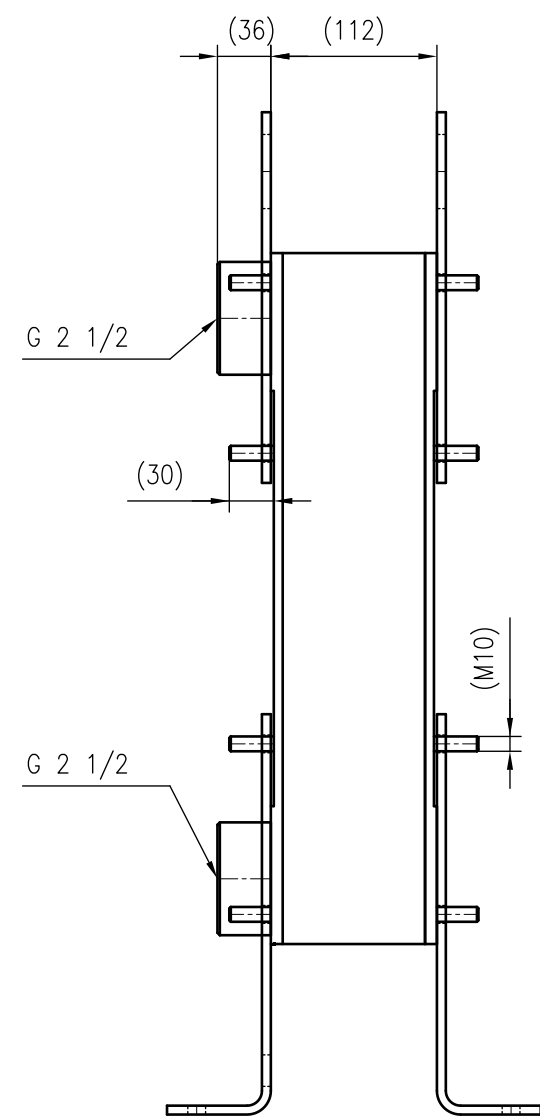
Side view
