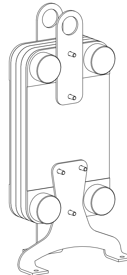
Isometric view
